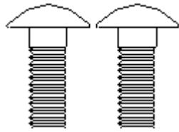
PART #82088 5/16-18 X 3/4" CARRIAGE BOLT Qty: 2
