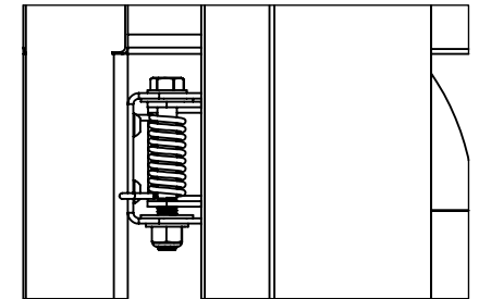
DETAIL A SCALE 1 : 4
