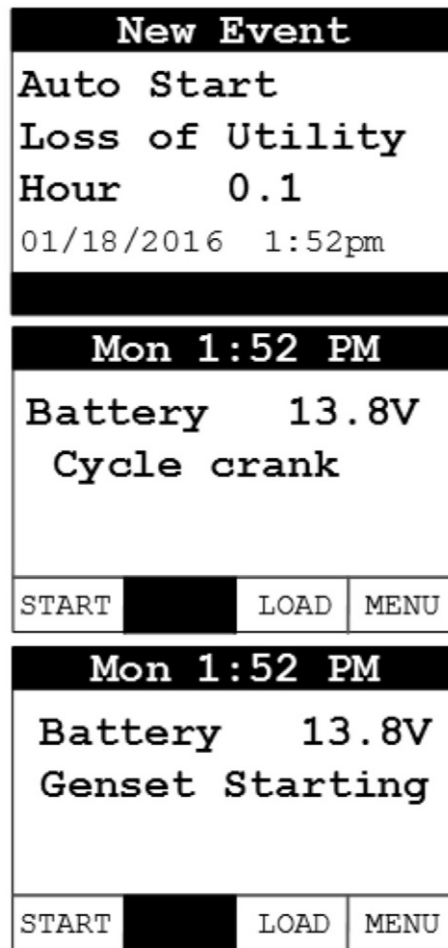
FIGURE 18. GENSET STARTING
