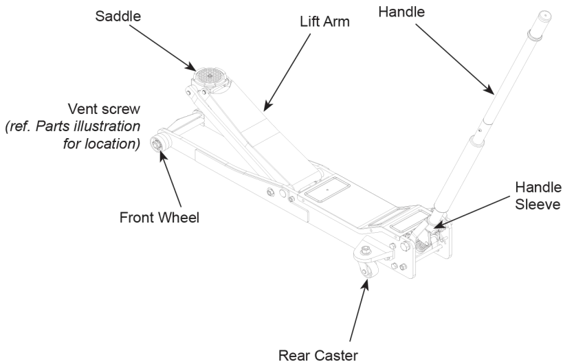
Figure 1 - Service Jack Nomenclature
