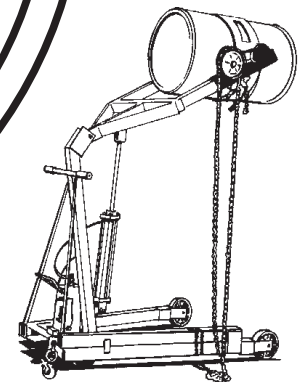
Drum Carrier/Rotator
