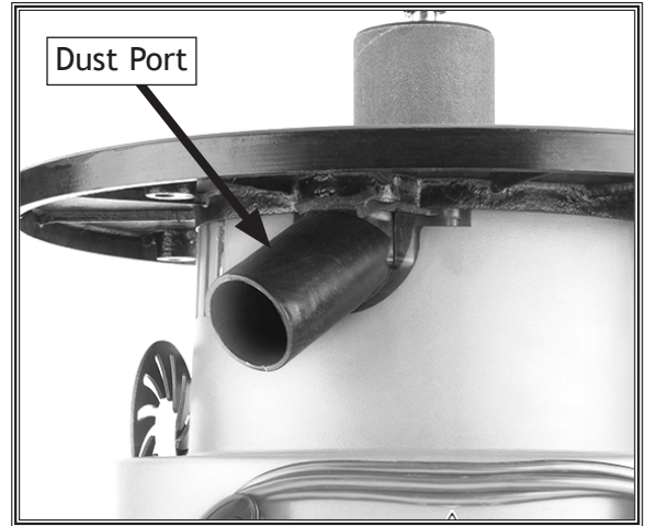
Figure 7. Location to install dust hose.
