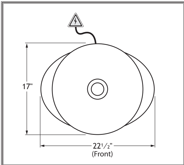
Figure 3. Machine clearances.
