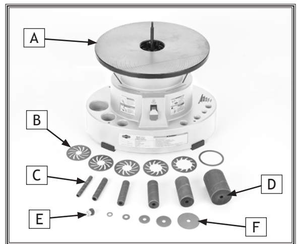
Figure 2. Spindle sander inventory.
