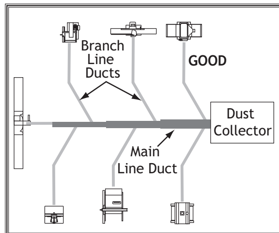
Figure 27. Efficient duct layout.
