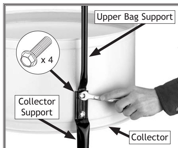
Figure 16. Mounting collector to brackets.
