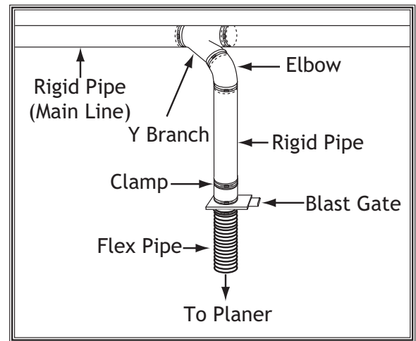
Figure 36. Drop down setup.
