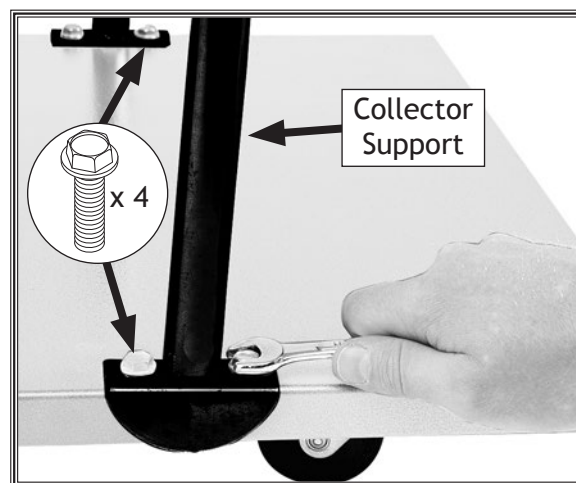
Figure 15. Installing collector support.
