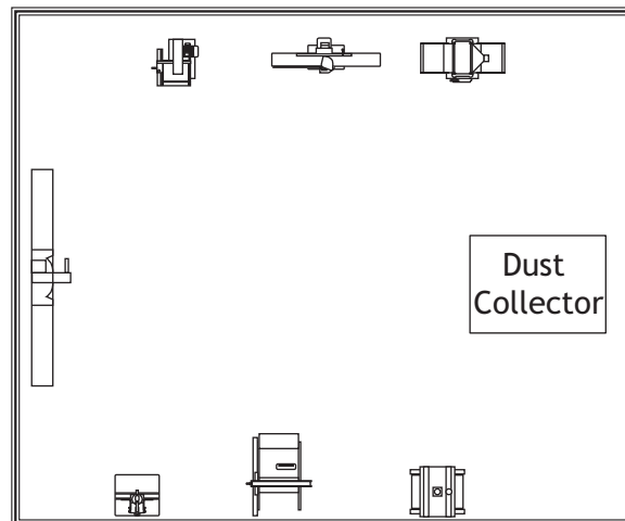
Figure 26. Basic sketch of shop layout.
