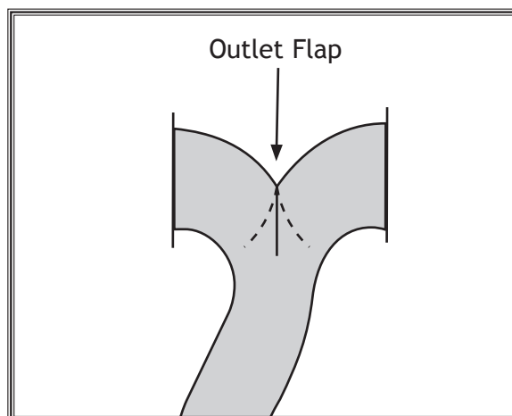
Figure 21. Outlet flap for equalizing filling of collection bags.
