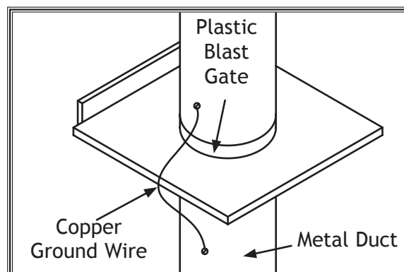
Figure 41. Ground jumper wire when using plastic blast gates and metal duct.
