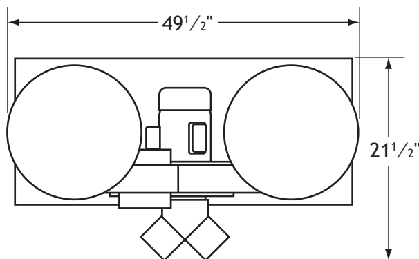
Figure 5. Working clearances.
