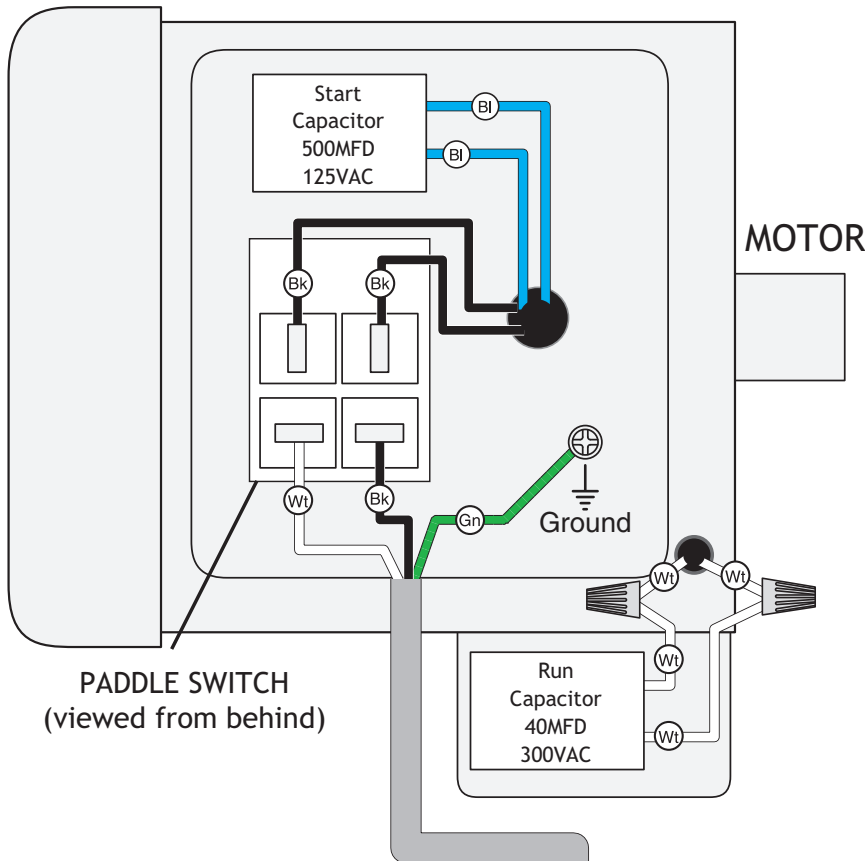
Figure 44. Junction box and start capacitor.
