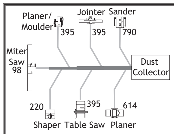
Figure 31. CFM requirements labeled.
