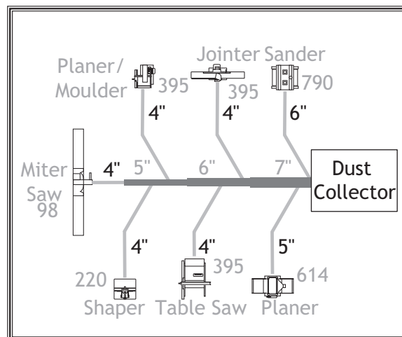
Figure 33. Branch line sizes labeled on sketch.
