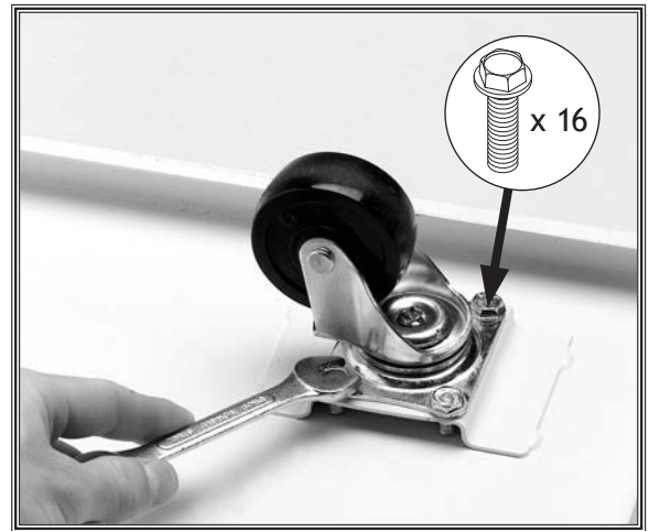
Figure 6. Installing caster to base.
