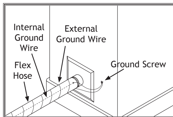
Figure 40. Flex-hose grounded to machine.
