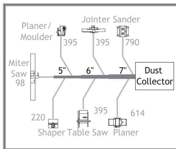
Figure 32. Main line size labeled on sketch.
