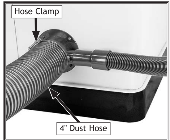
Figure 38. Dust hoses attached to port.
