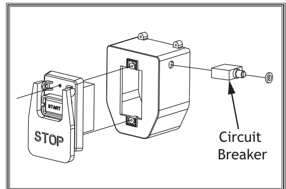
Figure 9. Location of circuit breaker.
