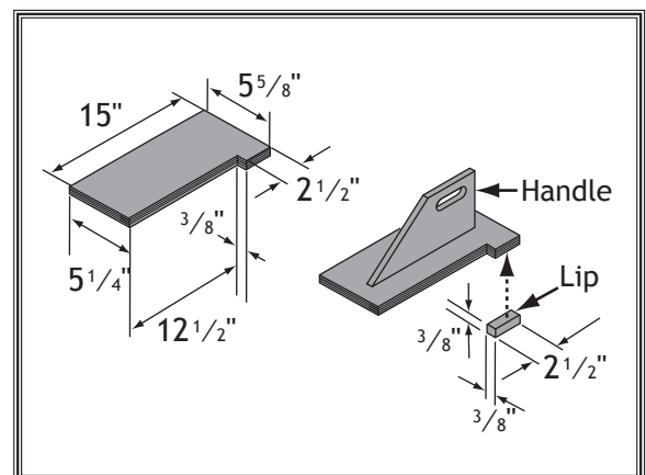
Figure 96. Push block dimensions and construction.
