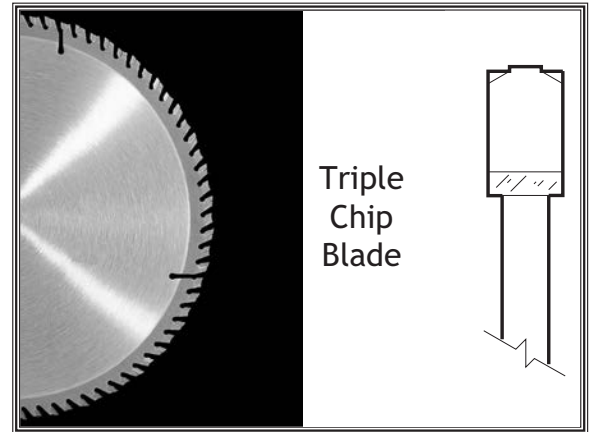
Figure 45. Example of a laminate blade.
