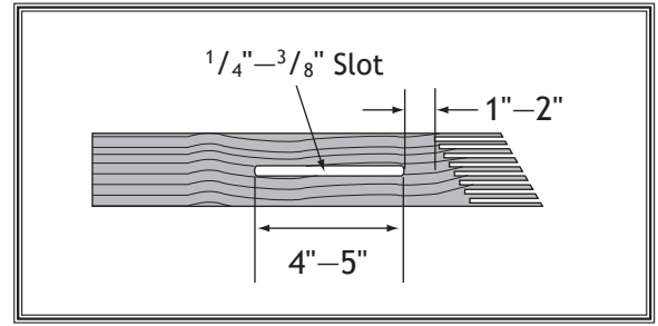
Figure 83. Slot routed in featherboard.
