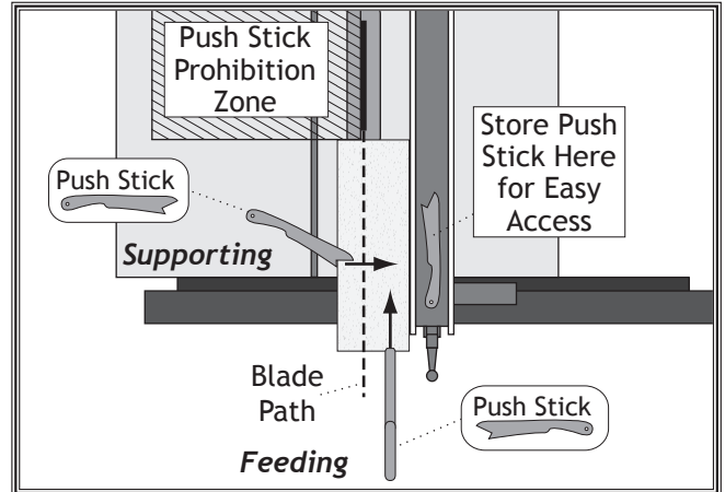
Figure 88. Using push sticks to rip narrow stock.
