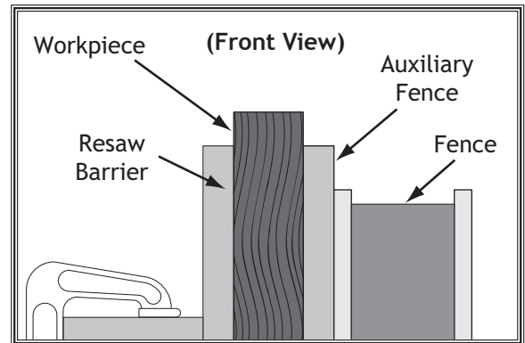
Figure 80. Example illustration of a resaw setup.
