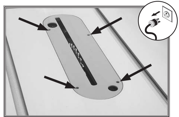
Figure 124. Location of table/dado insert holes with adjustment screws.
