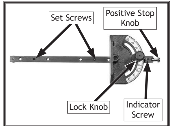
Figure 125. Set screws for adjusting miter bar in miter slot.
