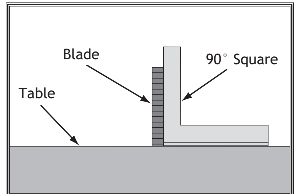
Figure 105. Checking blade at 90°.
