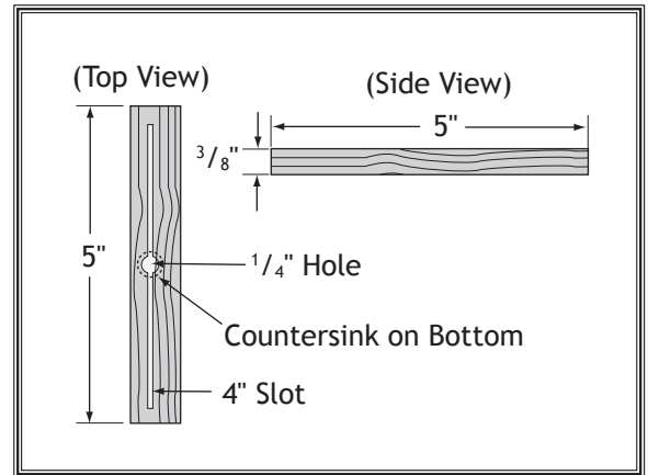
Figure 84. Miter bar pattern.
