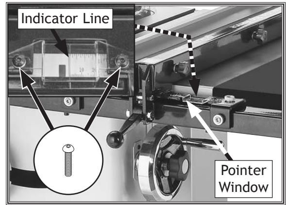
Figure 32. Aligning rail tape with scale pointer.
