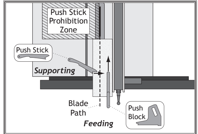
Figure 92. Using a push block and push stick to make a rip cut.
