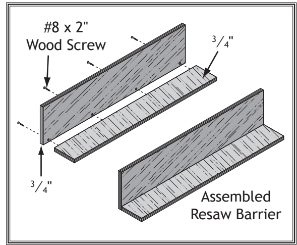
Figure 76. Resaw barrier.
