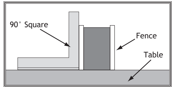
Figure 120. Checking if fence is square to table.
