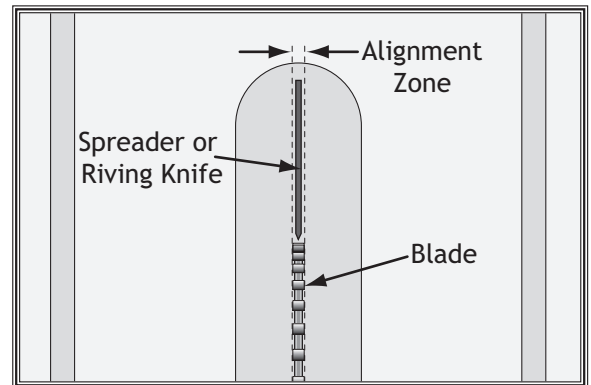
Figure 116. Spreader/riving knife alignment zone.
