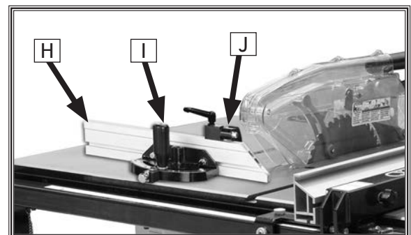
Figure 4. Miter fence and miter gauge.
