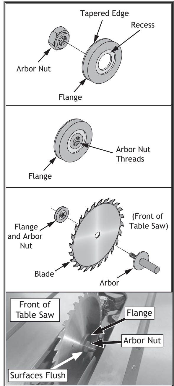
Figure 49. Blade order of installation and teeth facing correct direction.
