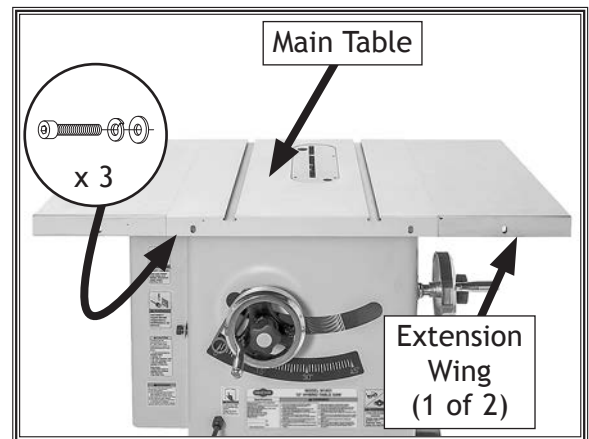
Figure 21. Extension wings installed.
