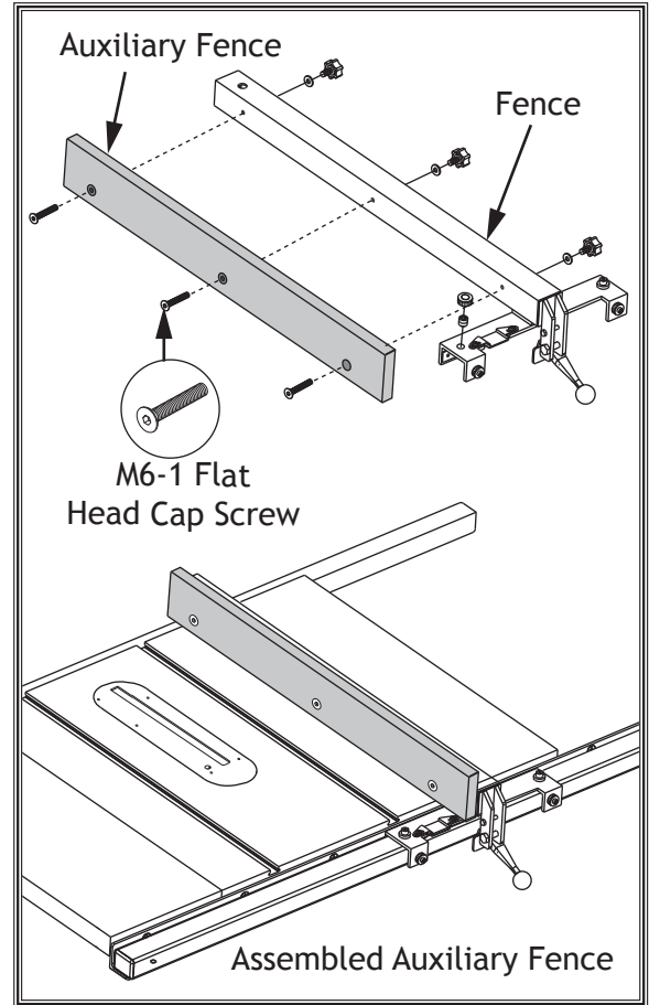
Figure 77. Example of auxiliary fence attached to Model W1851 fence face.
