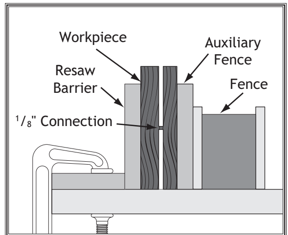
Figure 81. Ideal completed resaw operation.
