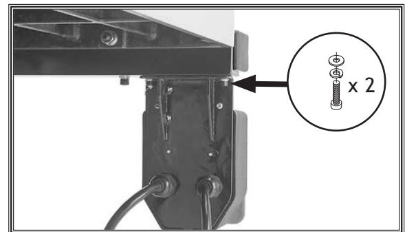
Figure 33. Switch installed.
