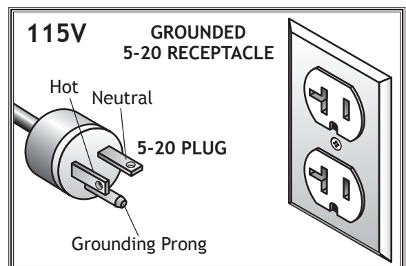
Figure 6. NEMA 5-20 plug & receptacle.
