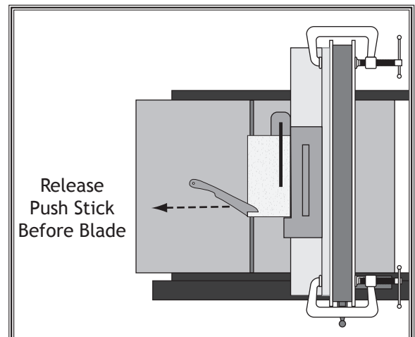
Figure 99. Ripping with push block.
