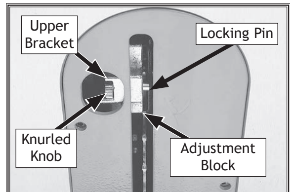
Figure 51. Knurled knob used to secure spreader.
