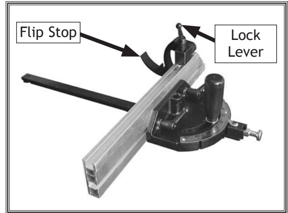
Figure 64. Location of flip stop lock lever.
