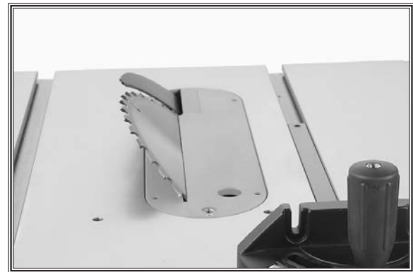
Figure 65. Blade tilted to 45° for bevel cutting on a typical table saw.
