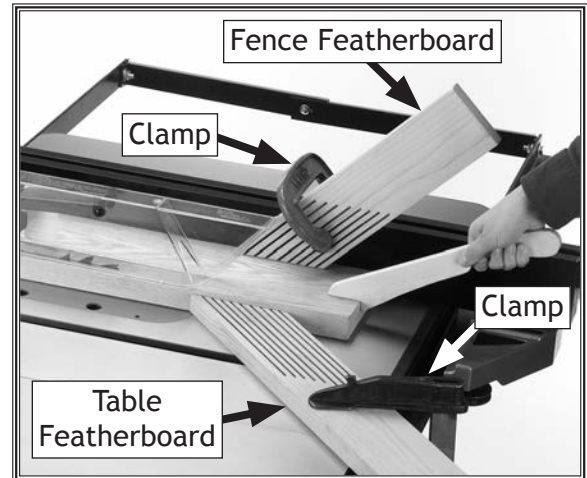
Figure 86. Example of featherboards secured with clamps.
