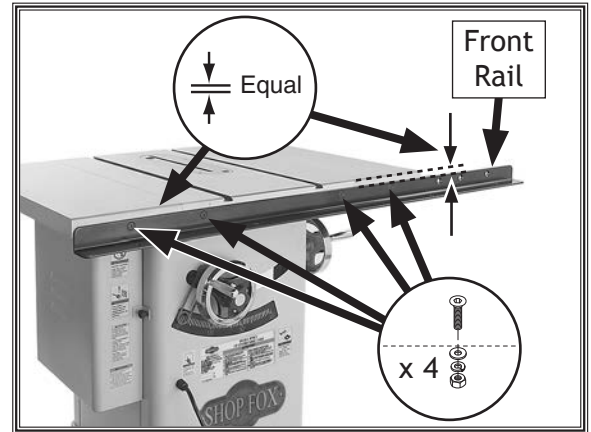
Figure 24. Front rail installed.
