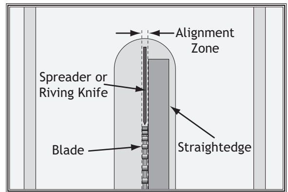
Figure 53. Spreader/riving knife alignment zone.
