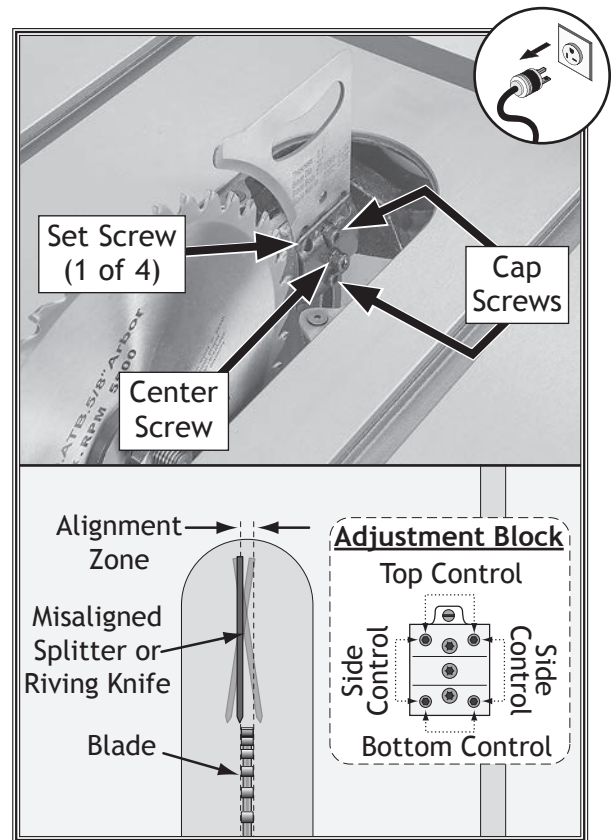
Figure 117. Set screws for adjusting spreader/riving knife position.
