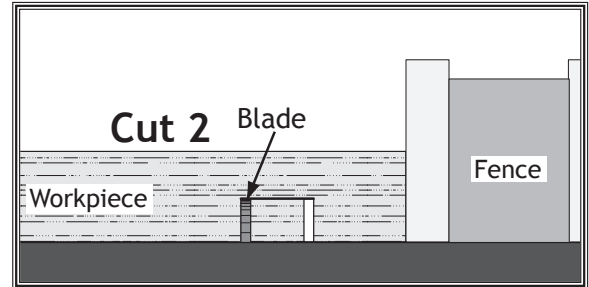
Figure 69. Second cut for a single-blade dado.
