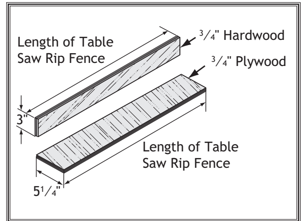
Figure 94. Auxiliary fence dimension.
