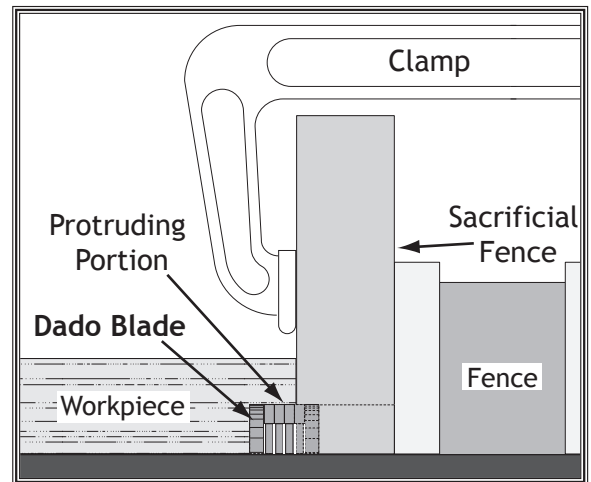
Figure 72. Rabbet cutting.
