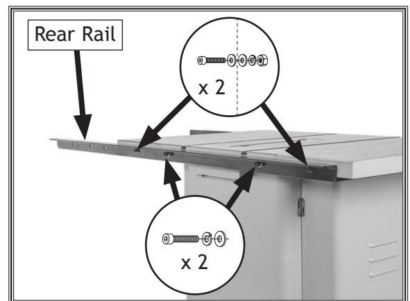
Figure 26. Rear rail installed.
