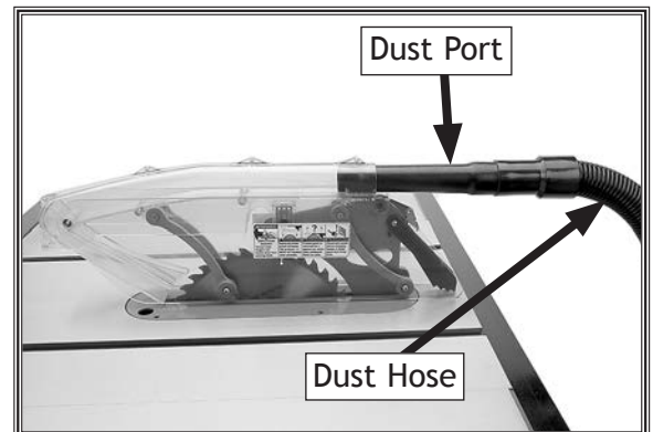
Figure 54. Dust port and dust collection hose installed on blade guard.
