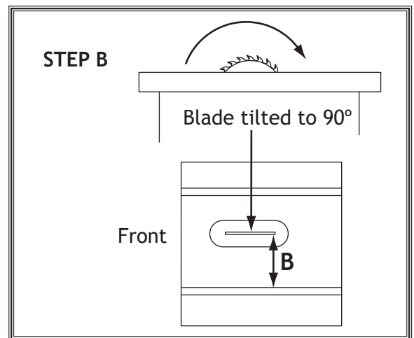
Figure 111. Making second slot-to-blade measurement at 90°.
