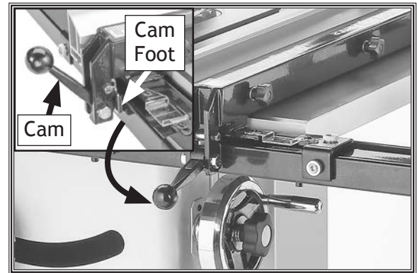
Figure 29. Fence installed on rails.
