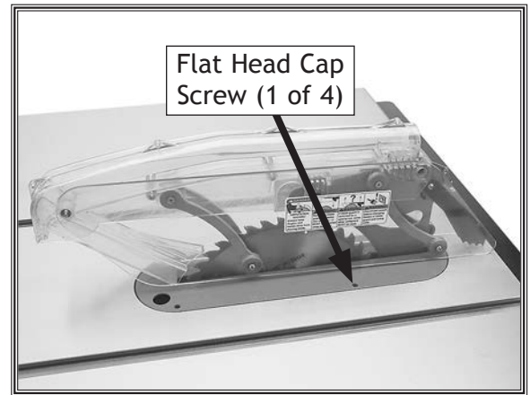
Figure 52. Blade guard installed.
