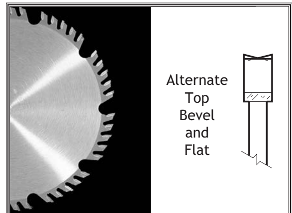
Figure 44. Example of a combination blade.
