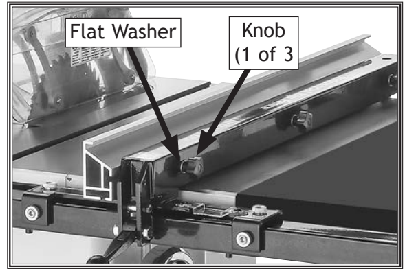
Figure 78. Location of knobs and flat washers securing fence to fence tube.
