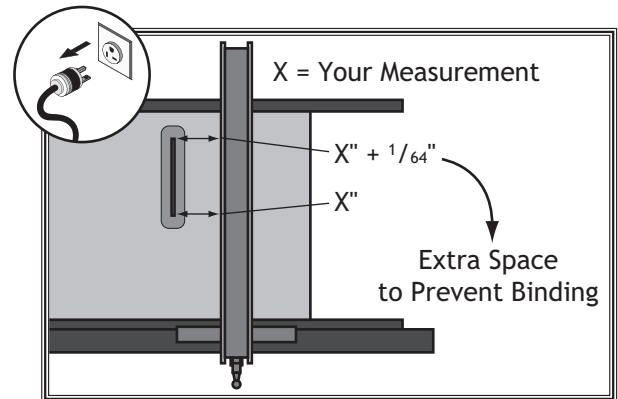
Figure 122. Adjusting fence with a \frac{1}{64} " offset.
