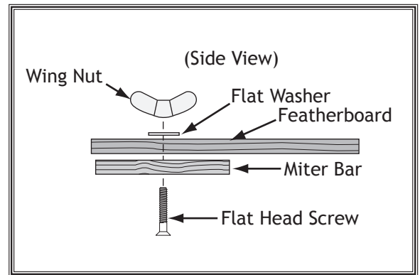
Figure 85. Assembling miter slot featherboard components.
