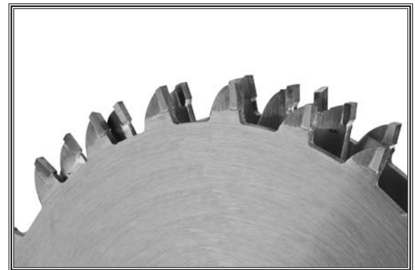
Figure 46. Stacked dado blade.
