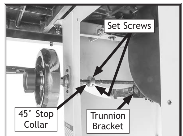
Figure 109. Location of 45° stop collar (right access cover removed).
