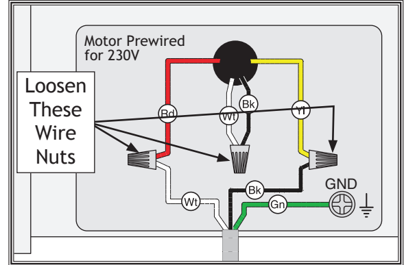
Figure 7. Location of wire nuts to be loosened on motor junction box.
