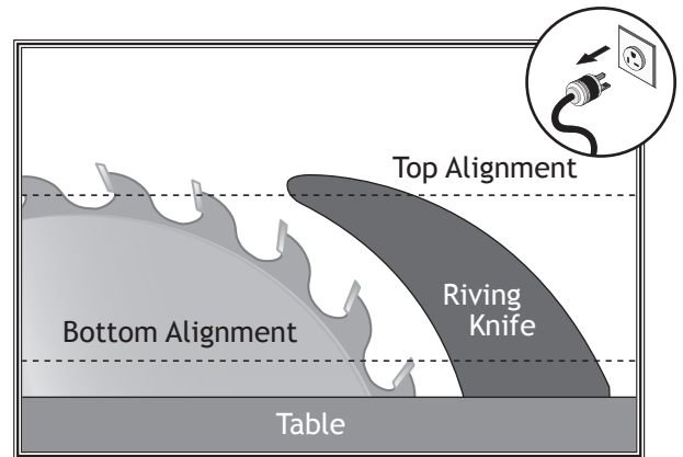
Figure 115. Example of checking top and bottom riving knife parallelism with blade.
