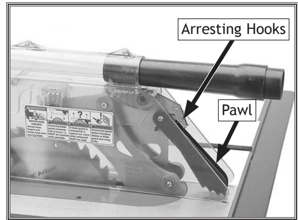
Figure 55. Pawls in resting position.
