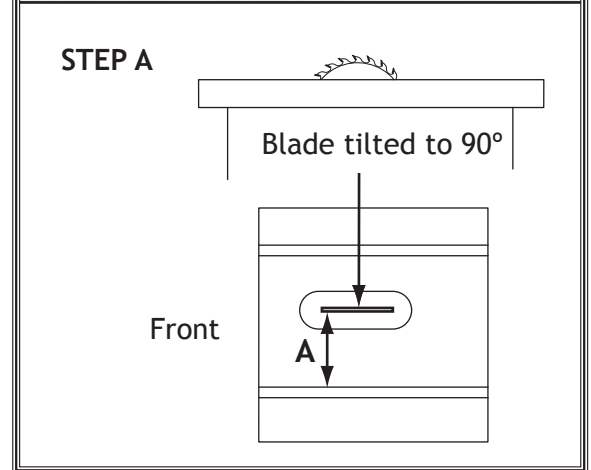
Figure 110. Making first slot-to-blade measurement at 90°.
