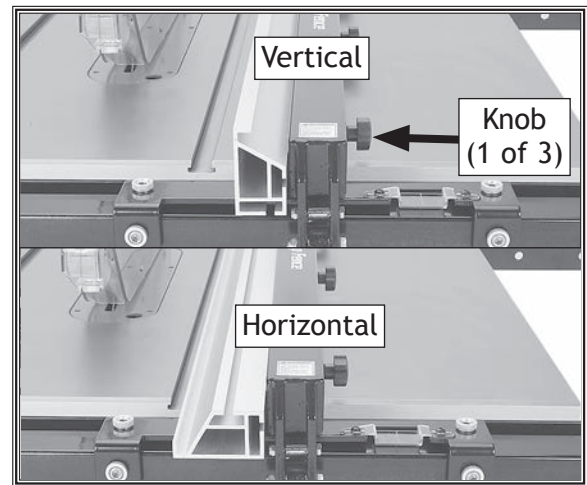
Figure 59. Rip fence positions.
