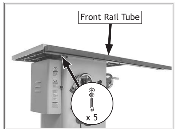
Figure 25. Front rail tube attached to front rail.
