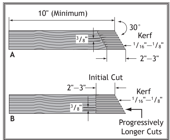
Figure 82. Patterns for making featherboards.
