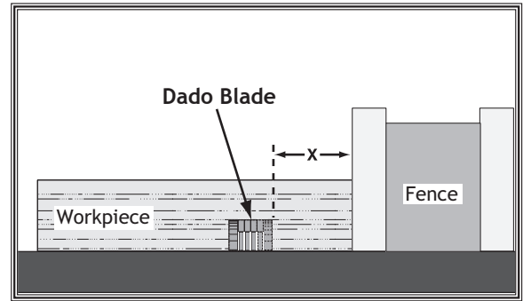
Figure 66. Example of a dado being cut with a dado blade.
