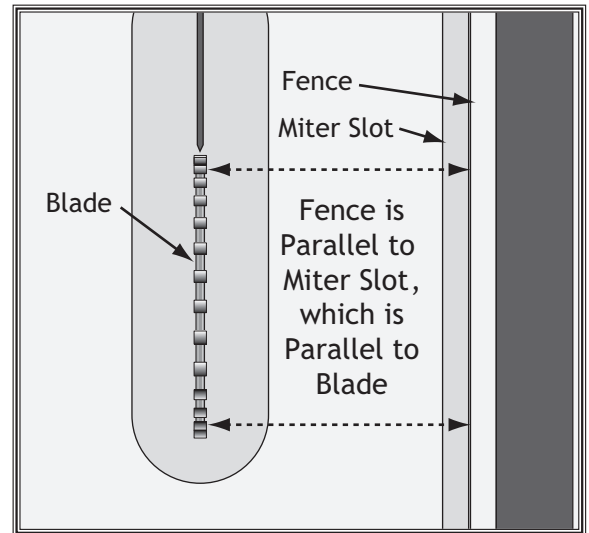
Figure 30. Checking fence parallelism with blade.
