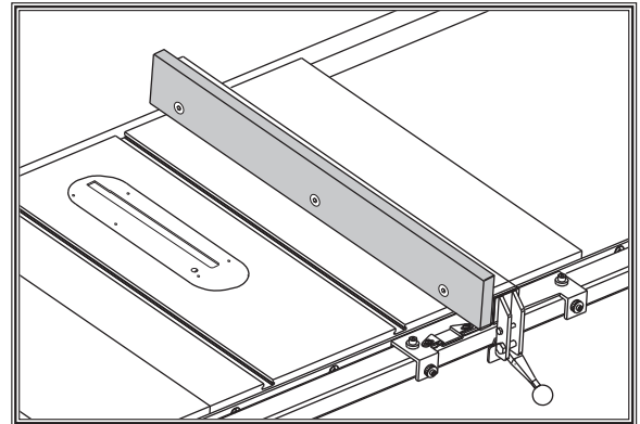
Figure 79. Example auxiliary fence attached to included fence.
