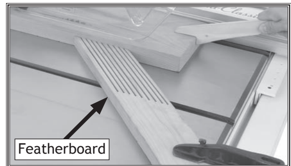
Figure 60. Typical ripping operation.
