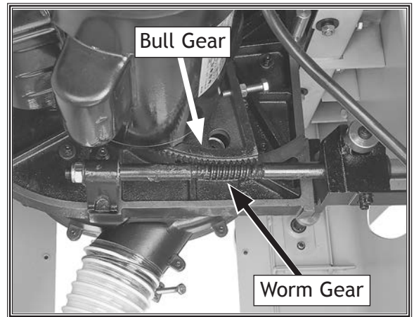
Figure 103. Worm and bull gear location.
