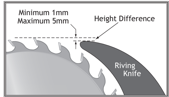
Figure 57. Example of height difference between riving knife and blade.
