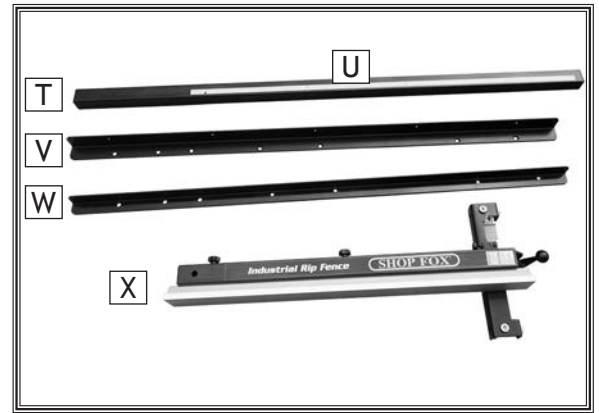
Figure 13. Inventory needed to install fence.
