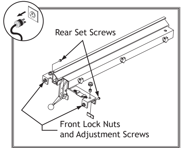
Figure 118. Location of screws used to adjust fence parallelism and clamping pressure.
