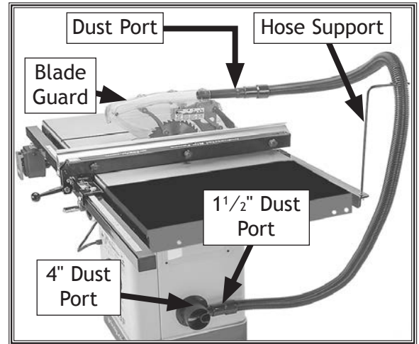
Figure 37. Dust hose attached to saw, hose support, and blade guard dust port.
