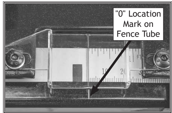
Figure 31. "0" location marked on fence tube.
