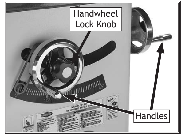
Figure 20. Handwheel installed.
