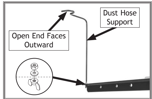
Figure 34. Dust hose support installed.
