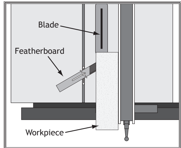
Figure 87. Featherboard installed in miter slot and supporting workpiece for ripping cut.
