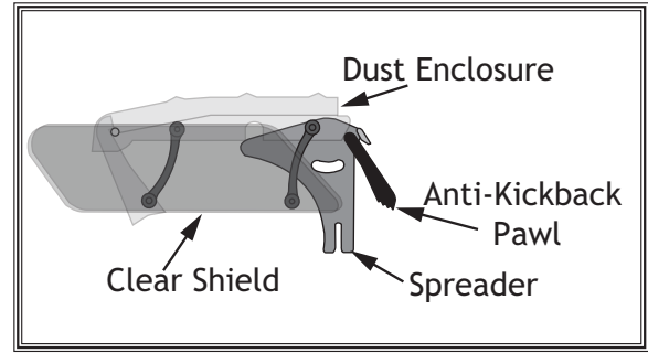
Figure 50. Blade guard assembly components.
