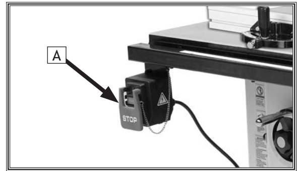
Figure 1. Location of START/STOP switch.
