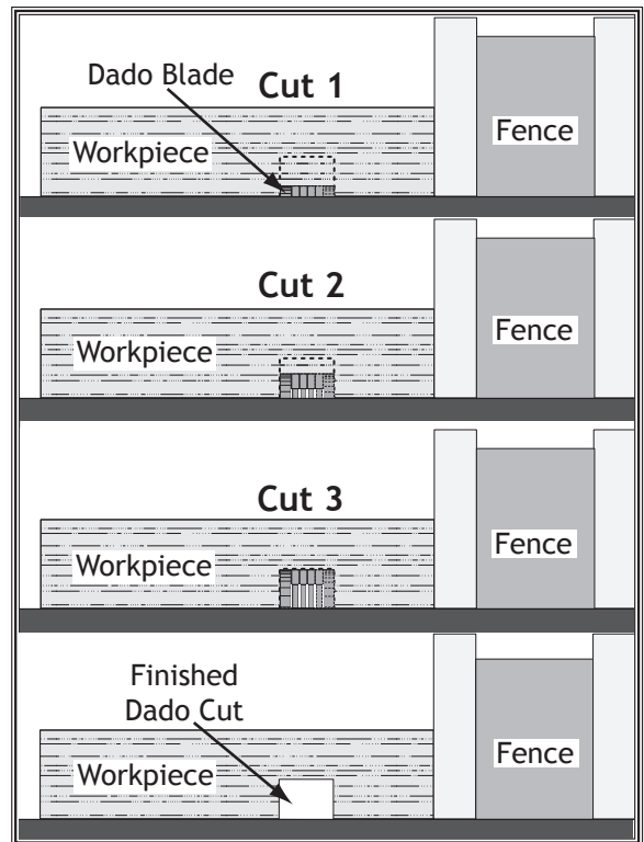
Figure 67. Example of dado being cut with multiple light cuts, instead of one deep cut.
