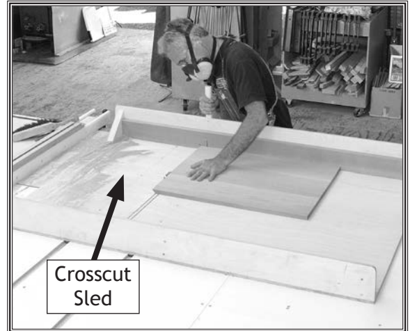
Figure 101. Example of a crosscut sled.
