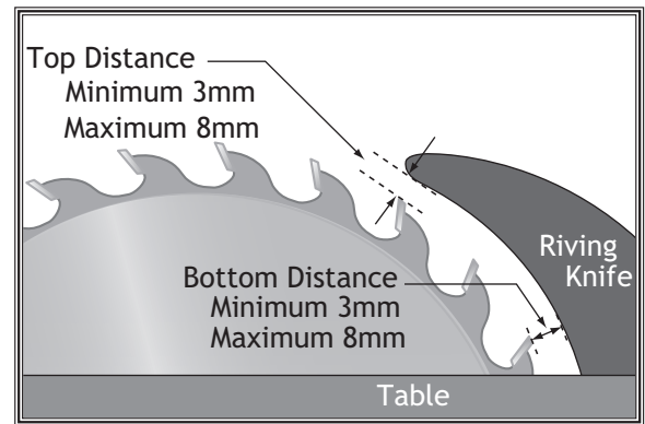
Figure 58. Example of allowable top and bottom distances between riving knife and blade.
