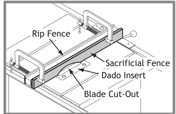
Figure 71. Example of sacrificial fence.
