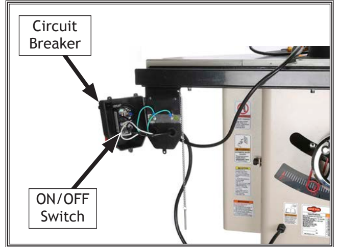
Figure 132. Switch box components.
