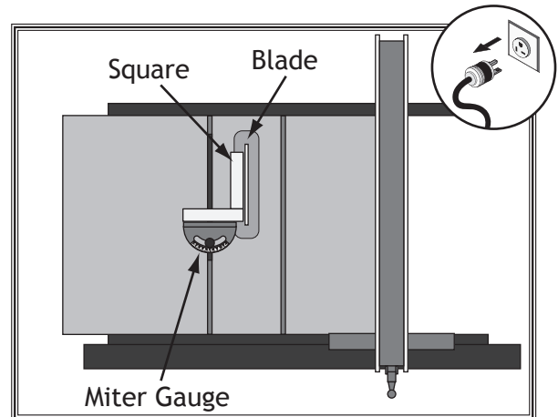
Figure 126. Checking 90° stop on miter gauge.
