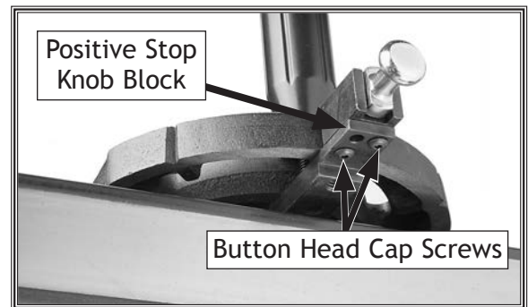
Figure 127. Screws for adjusting miter body.
