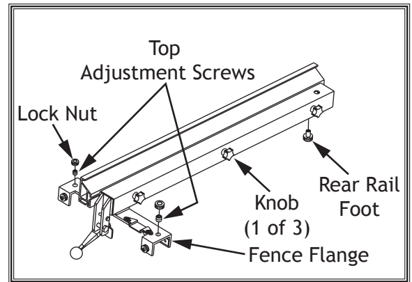
Figure 119. Fence components used to adjust fence height and squareness to table.
