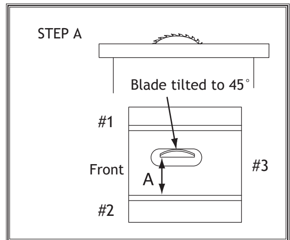
Figure 113. Shim procedure diagram A.
