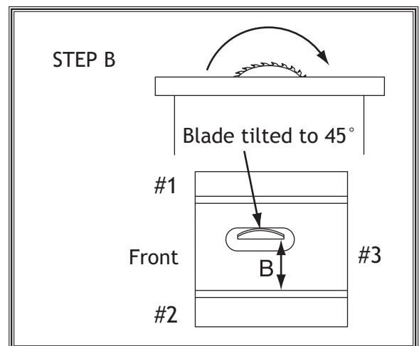
Figure 114. Shim procedure diagram B.
