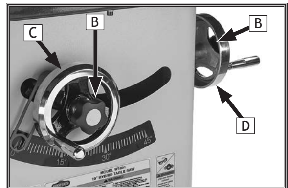
Figure 2. Blade adjustment handwheels and locks.
