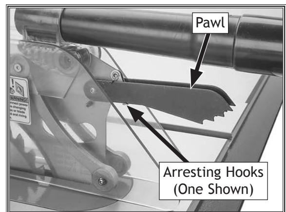
Figure 56. Pawls disabled.
