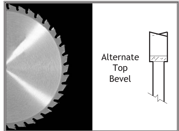
Figure 43. Example of a crosscut blade.
