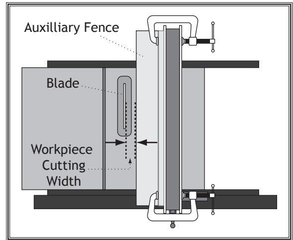
Figure 97. Adjusting ripping distance between blade and auxiliary fence.
