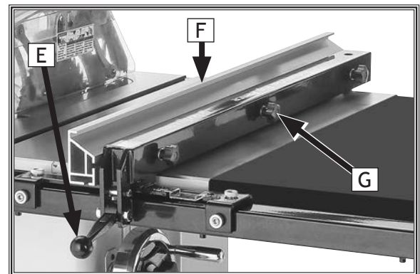
Figure 3. Location of fence controls.
