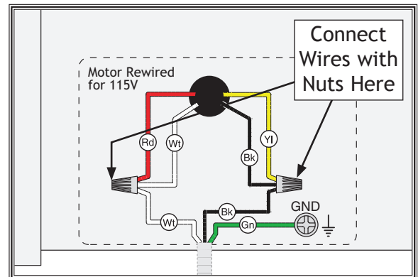
Figure 8. Motor rewired to 115V.
