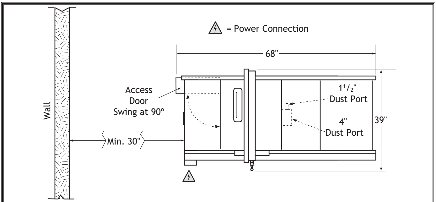
Figure 16. Working clearances.
