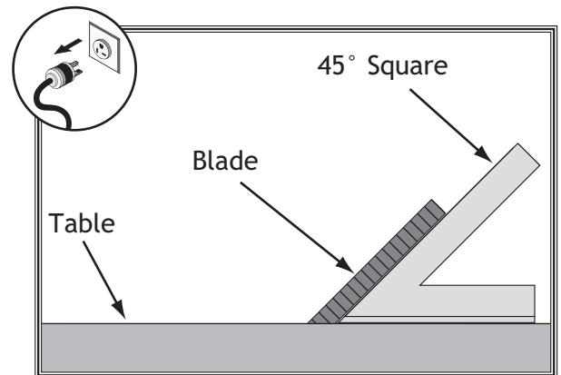
Figure 108. Checking blade at 45°.
