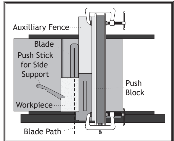
Figure 98. Push block in position to push workpiece through blade.
