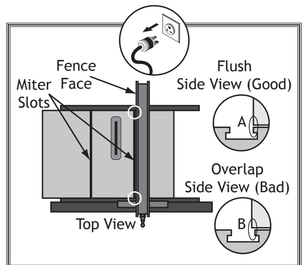
Figure 121. Example of aligning fence to miter slot.
