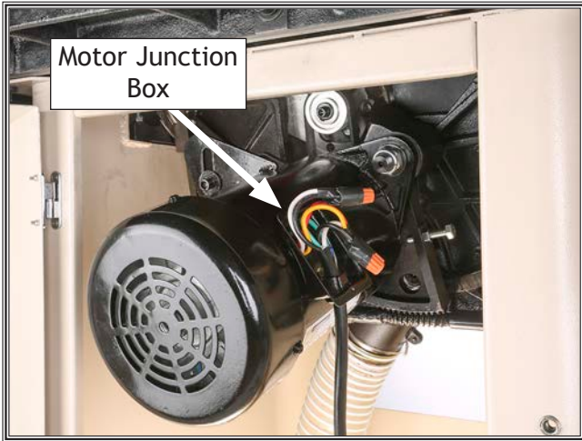
Figure 131. Motor junction box.
