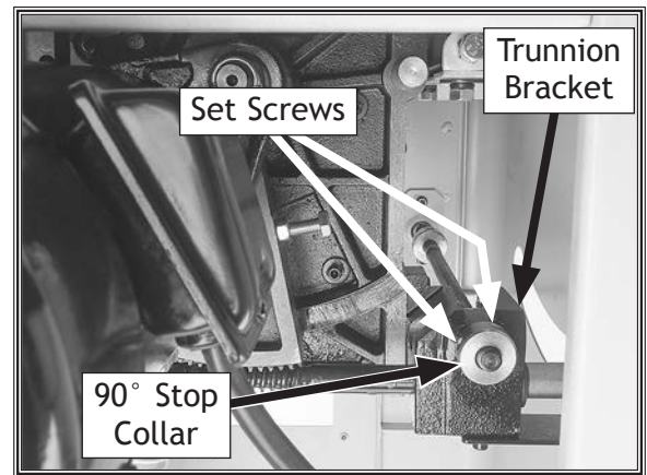
Figure 107. 90° stop collar and set screws.
