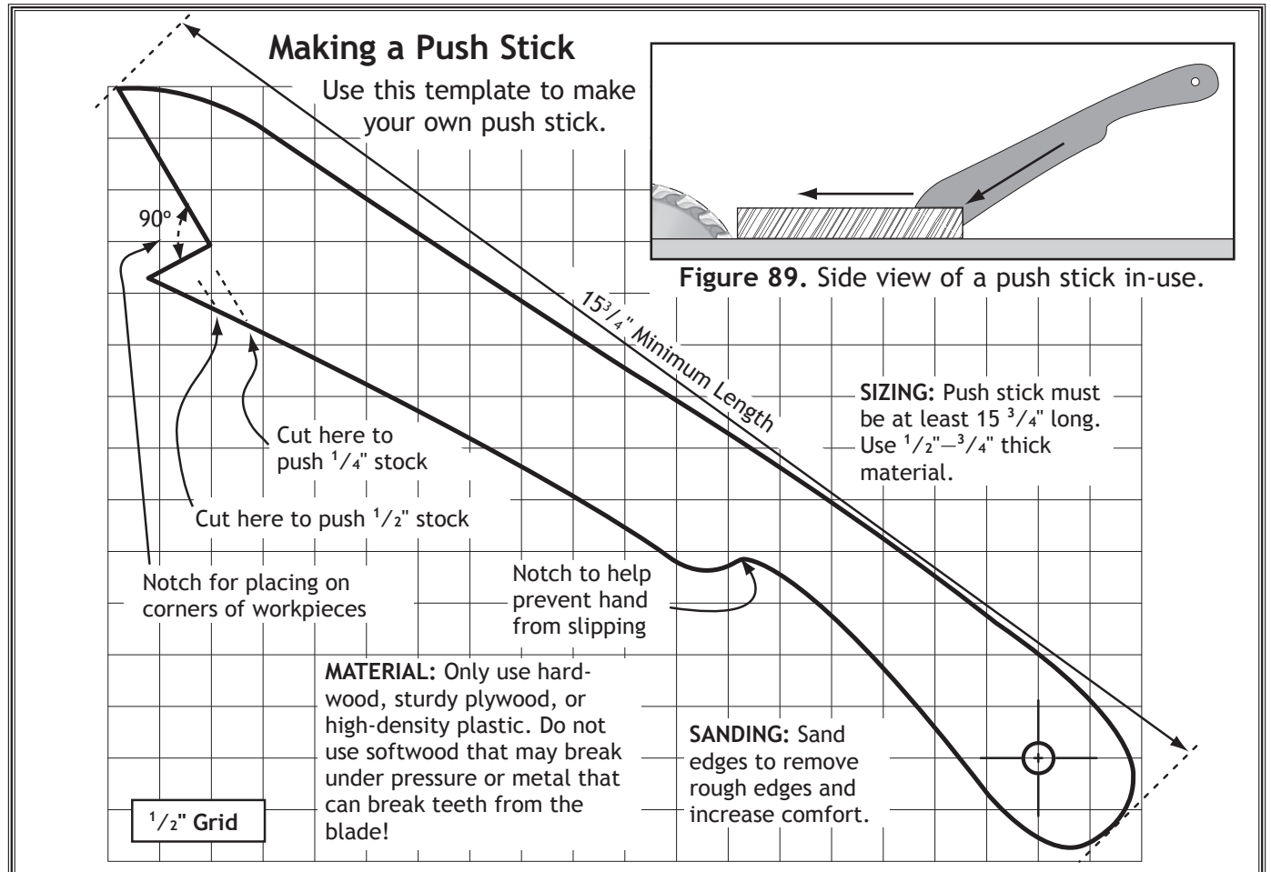
Figure 90. Template for a basic shop-made push stick (not shown at actual size).
