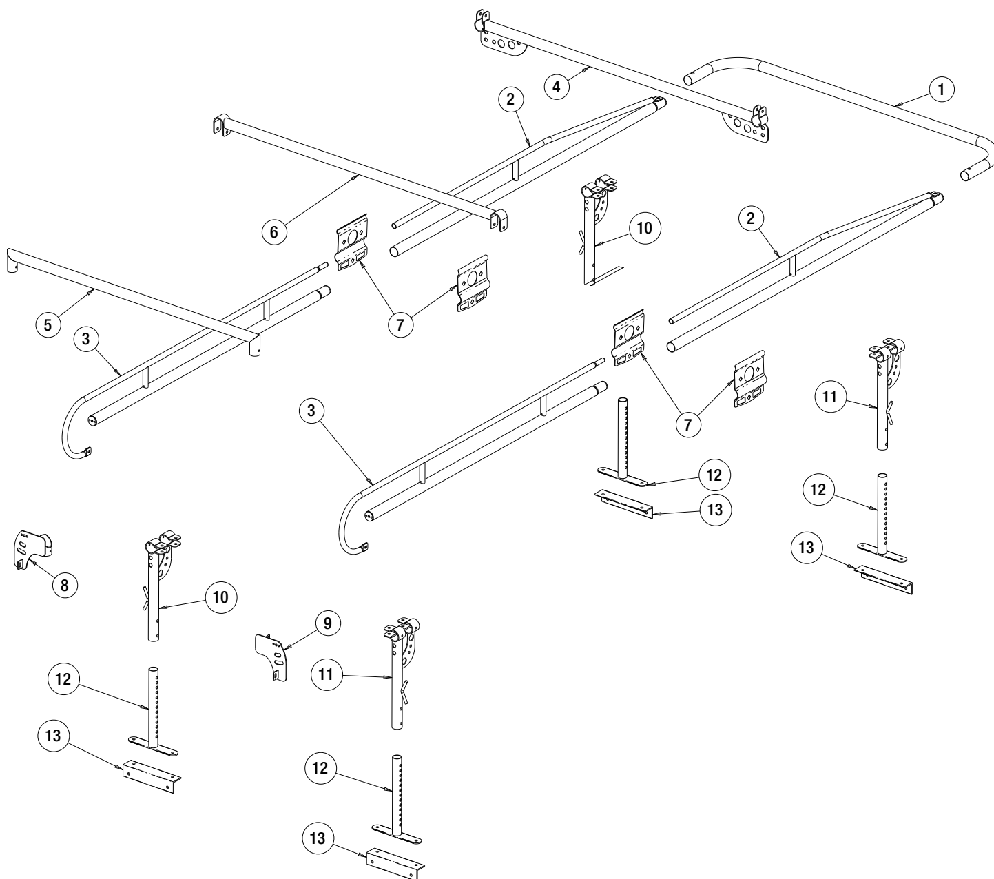
Fig. 5 - PARTS
