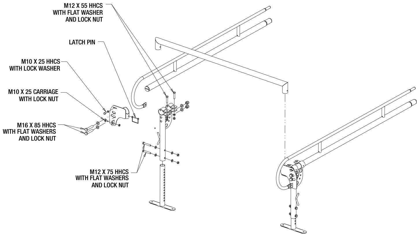
Fig. 2 - REAR RAIL, CROSSBAR AND FEET
