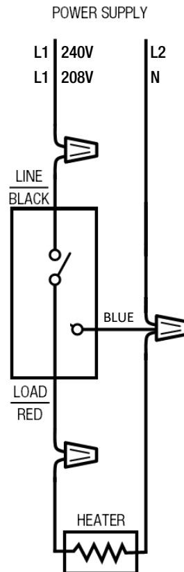
K901-DB-B / K901-DB-W wiring diagram:
