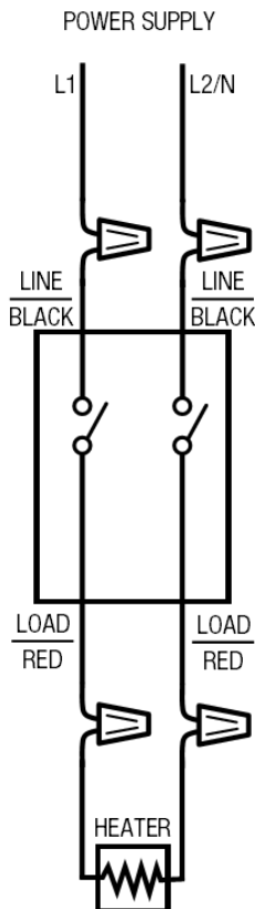
K902-DB-B / K902-DB-W wiring diagram:
