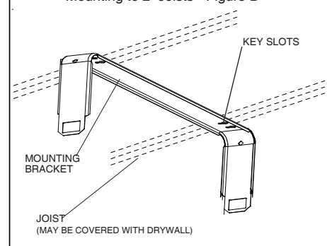
Mounting to 2 Joists - Figure B
