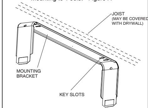
Mounting to 1 Joist - Figure A
