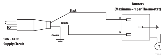
FIGURE 17: Ener-Radiant XL Burner Internal Wiring
