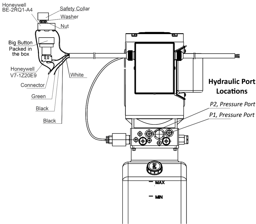
Electrical Schematic
