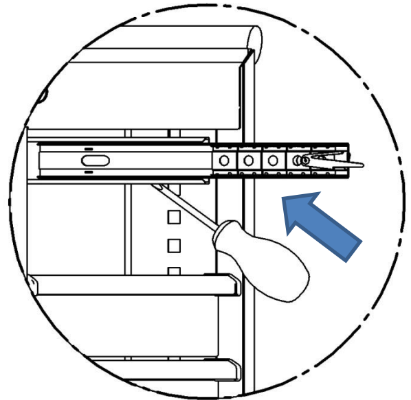
Detail G
