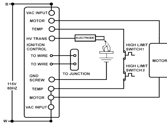
SCHEMATIC DIAGRAM
