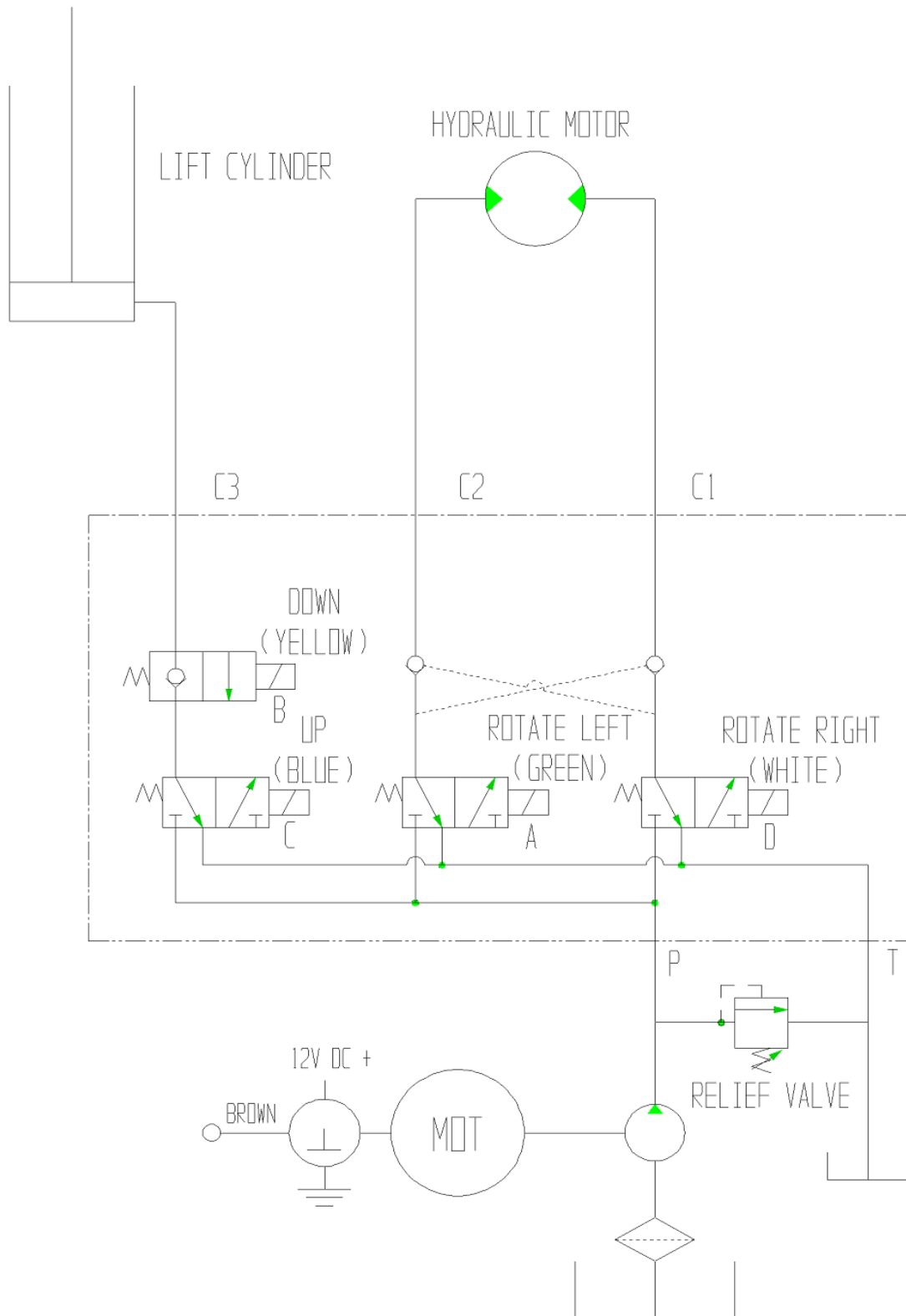
HYDRAULIC SCHEMATIC
