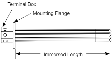
Flanged Immersion Heater
