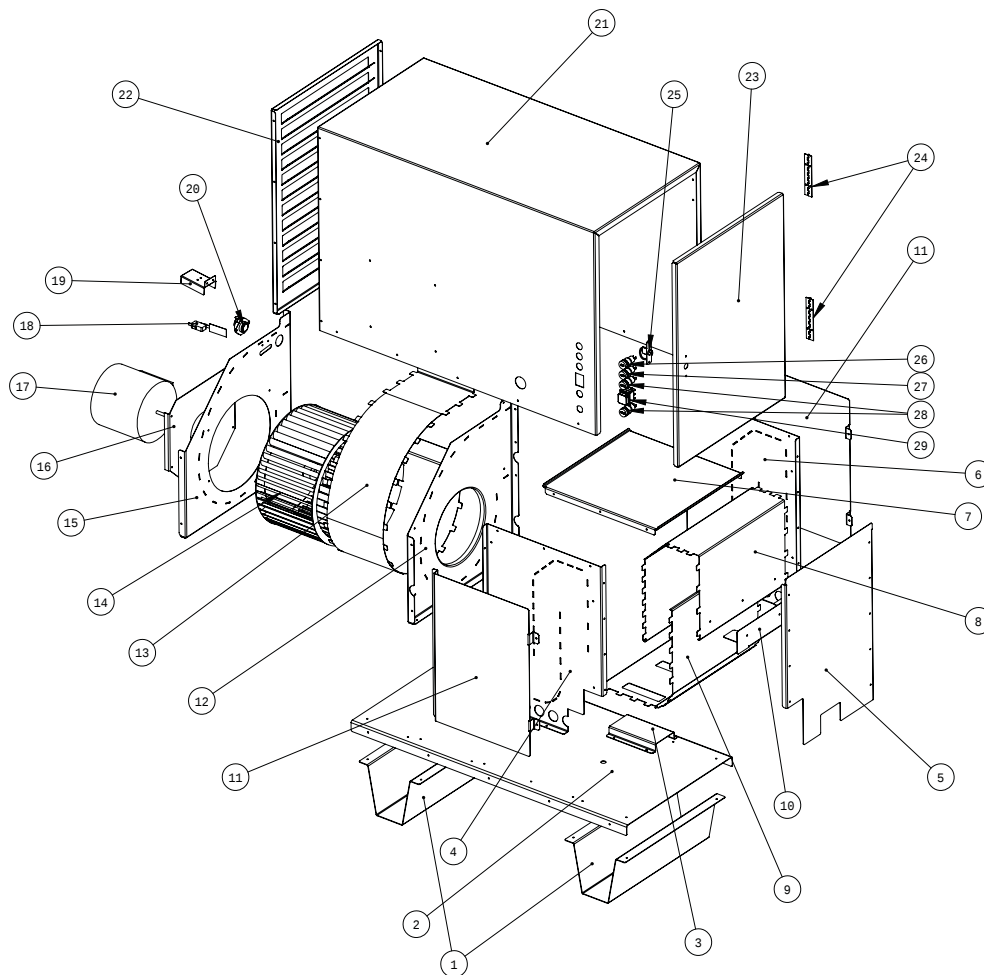
EXPLODED VIEW HS115TC
