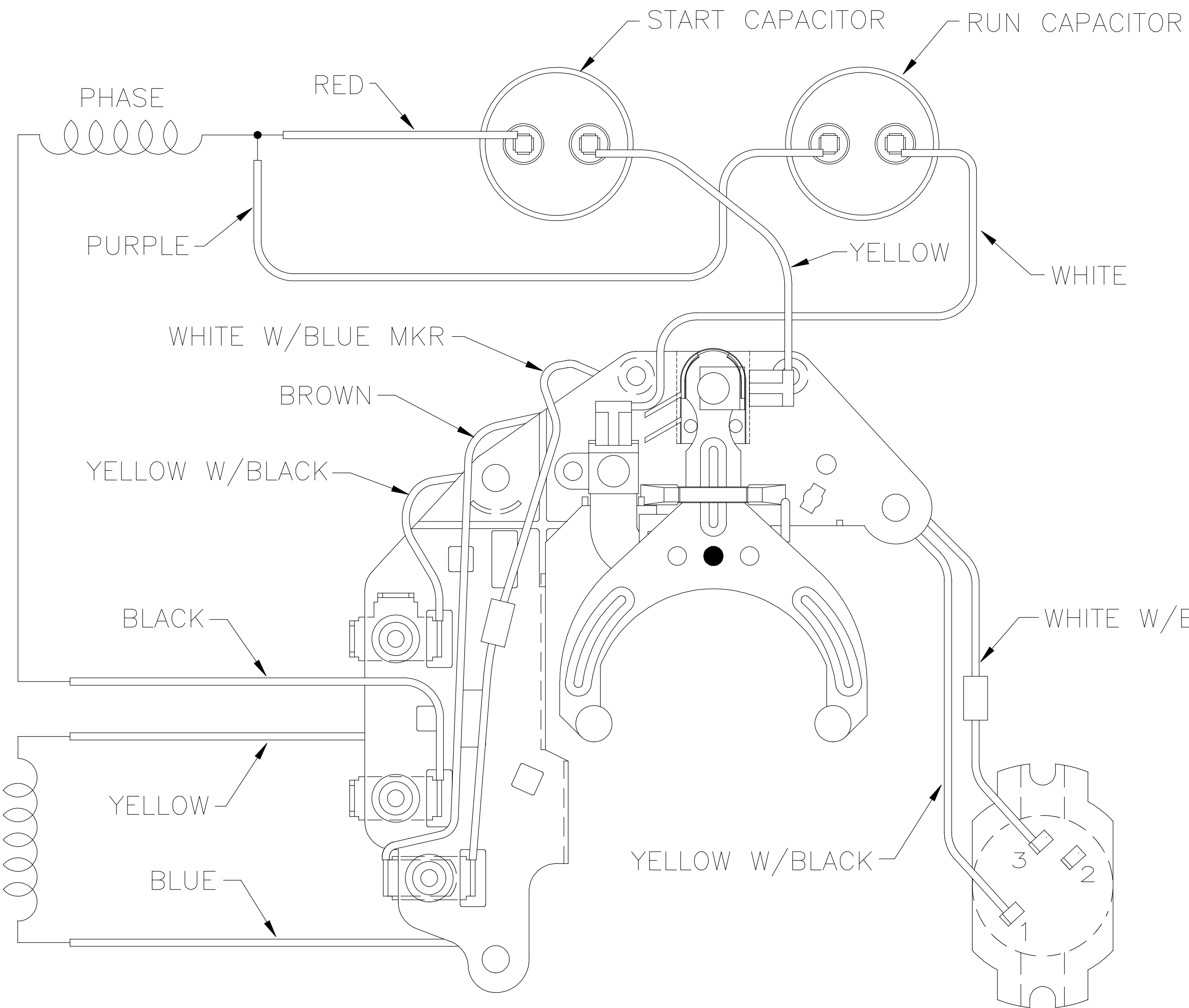
INTERNAL CONNECTIONS
