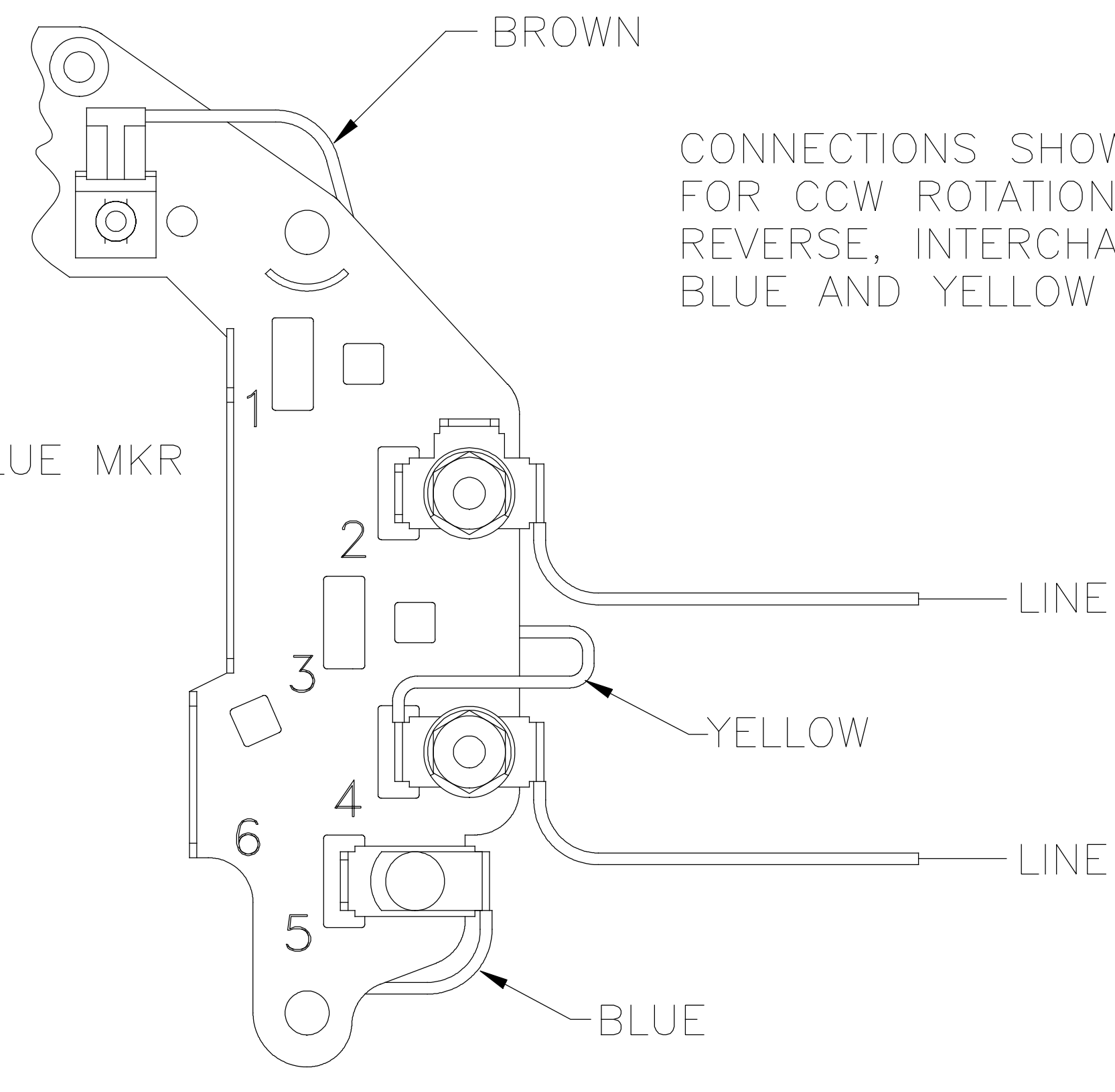
EXTERNAL CONNECTIONS
