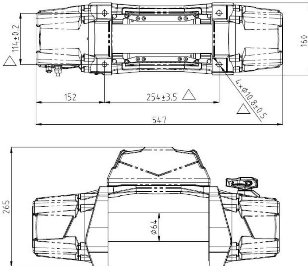
Figure D: winch dimensions
