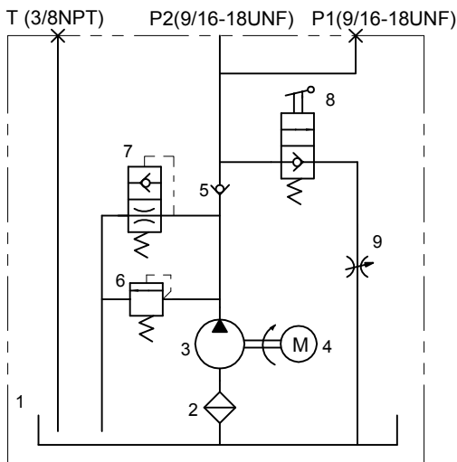
Hydraulic Schematic
