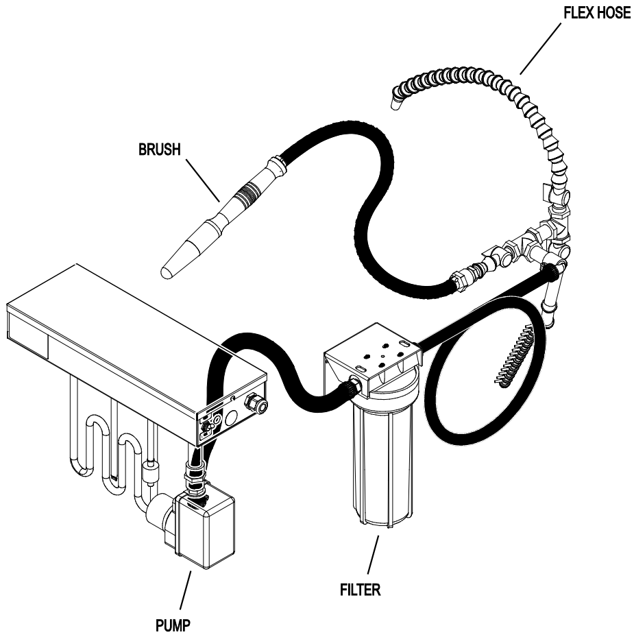
Fluid Flow
