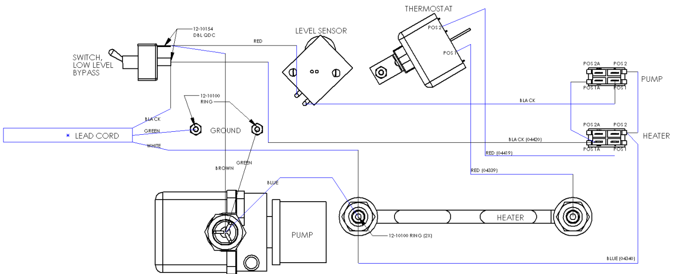
WIRING DIAGRAM
