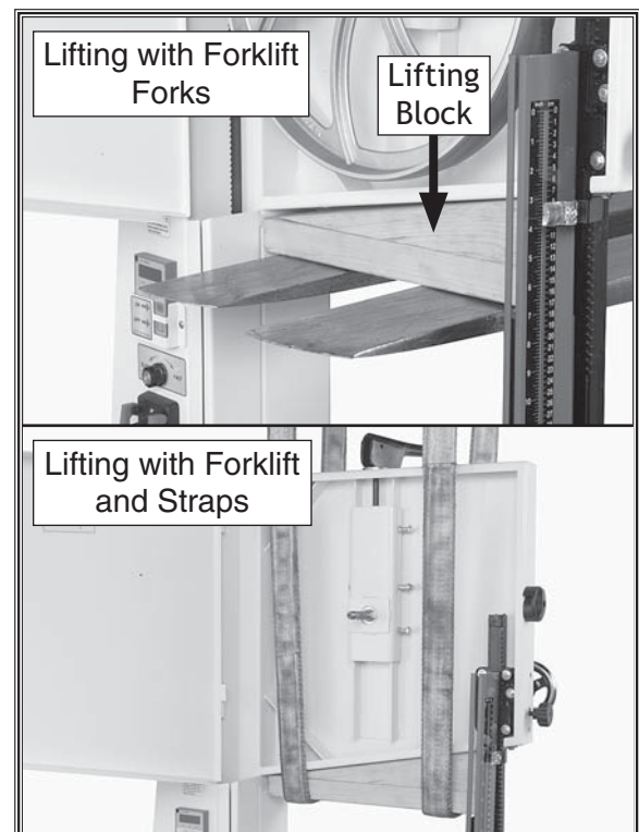
Figure 6. Lifting machine with a forklift.
