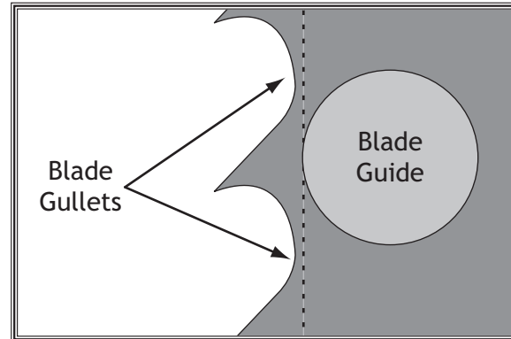
Figure 29. Lateral adjustment of blade guides.
