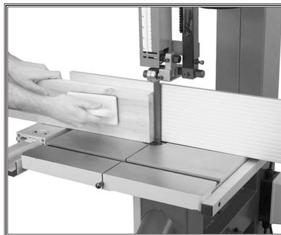
Figure 42. Typical resawing operation.
