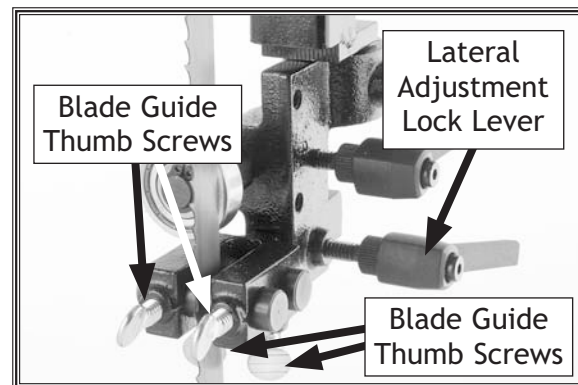
Figure 28. Blade guide controls.
