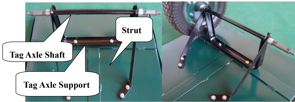
Figure 1. Tag Axle and Wheel Installation
