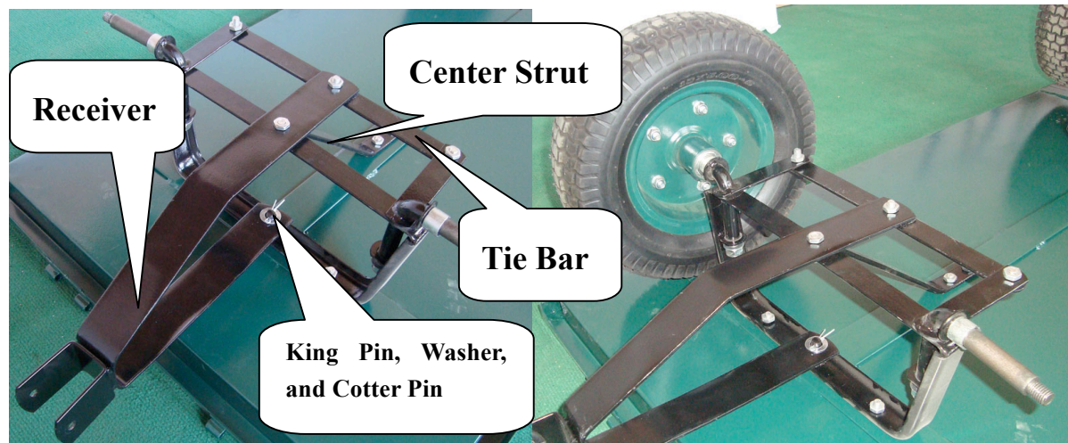
Figure 2. Steering Axle
