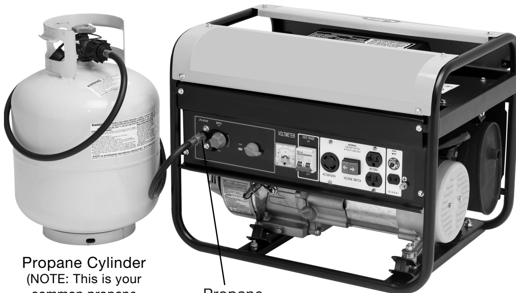
Propane Intake Valve
