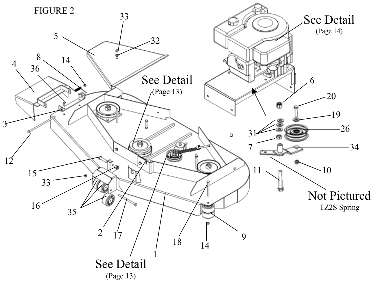
DECK ASSEMBLY FIGURE 2
