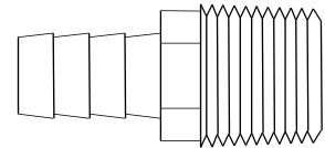
1/2" MPT x 1/2" Hose Barb 777445
