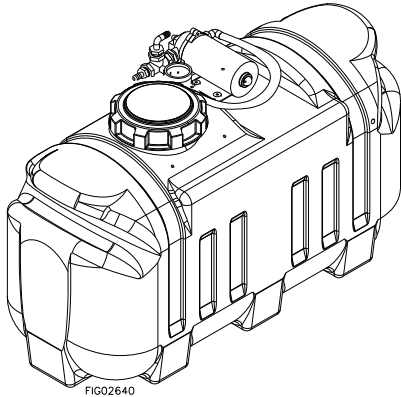
Sprayer
