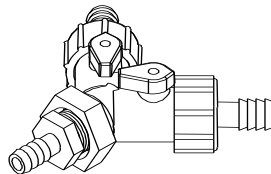
Boom Valve Assembly 5232 (Qty 2) Rubber Washer 5222 (Qty 1) 3/4" GHT x 1/2" Hose Barb 5212 (Qty 2) 1/2" Flat Seat Hose Barb 777850 (Qty 2) 3/8" GHT Swivel 777849 (Qty 1) Boom Valve
