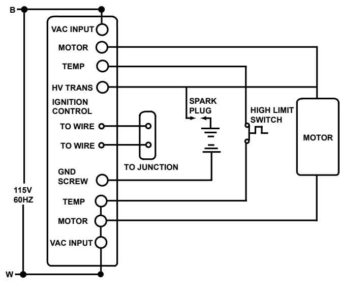
SCHEMATIC DIAGRAM
