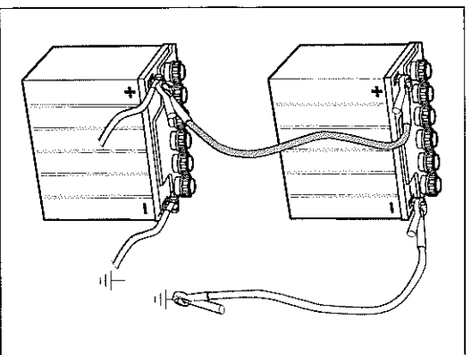
Jumper cable connection
