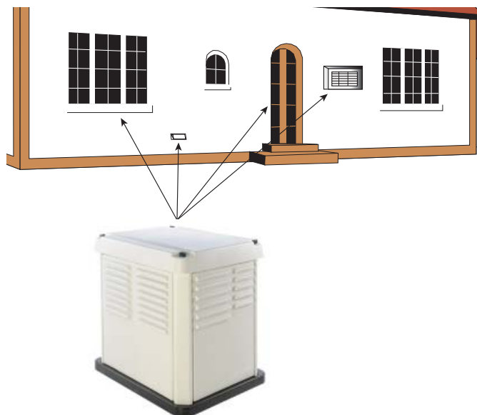
Figure 1.6 – Generator Clearances
