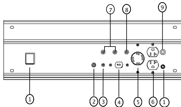
Operation Panel
