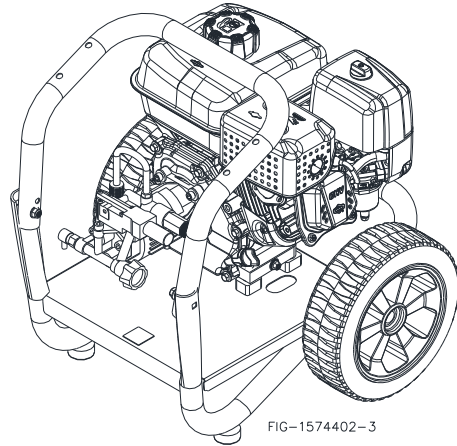
Engine/Pump/Base Assembly
