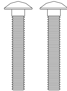
BOLT, CARRIAGE GR5Z 5/16"-18X2" PW QTY 2 PART# 82233
