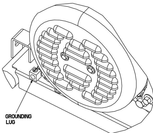
Figure 16 - Grounding the Generator
