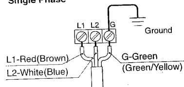
Single Phase
