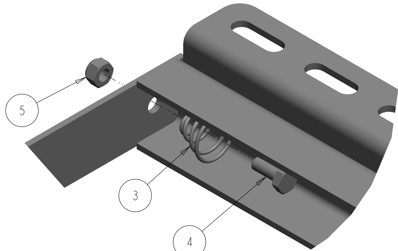
2X SPRING INSTALLATION DETAIL A SCALE 1.000
