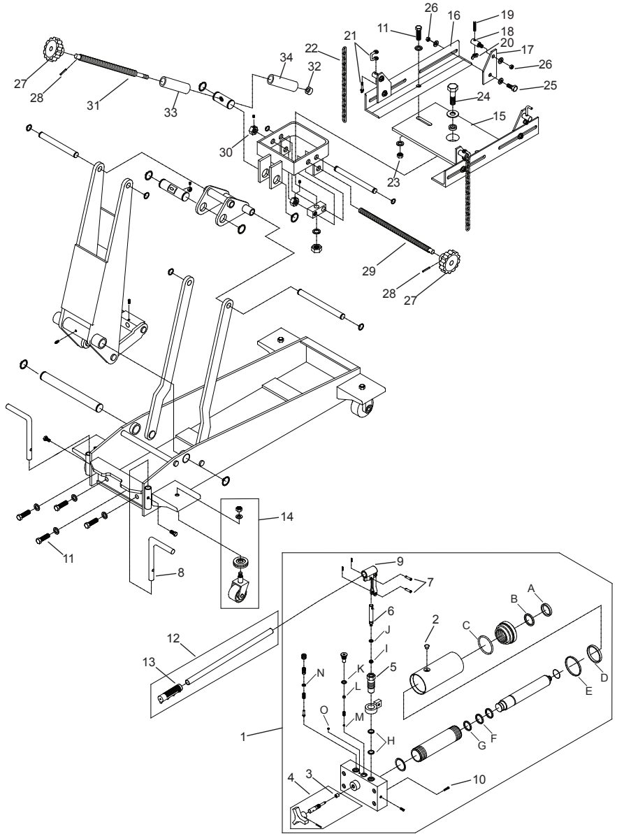
Figure 5 - Replacement Parts Illustration for Model 42000C
