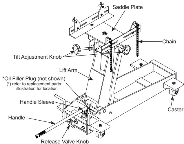
Figure 1- Typical Transmission Jack Components (42000C shown)
