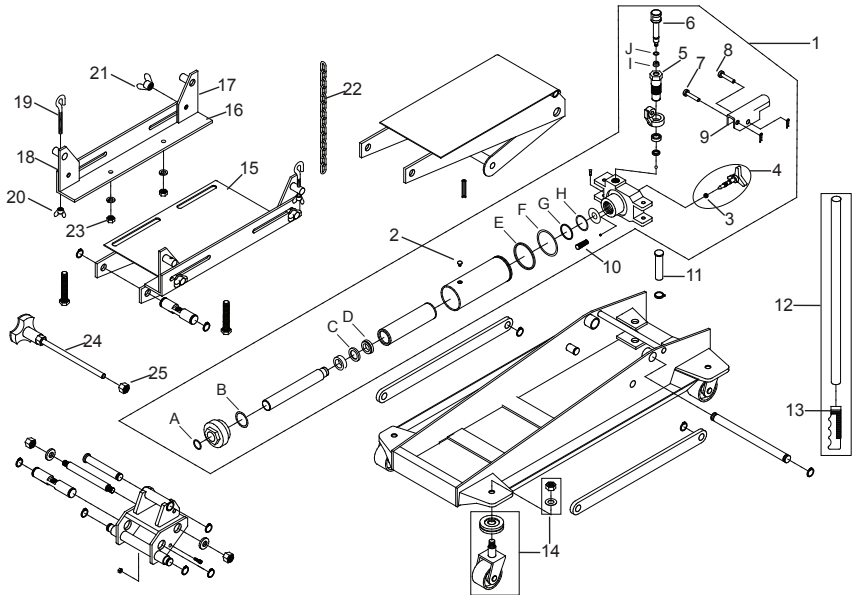
Figure 4 - Replacement Parts Illustration for Model 41100C
