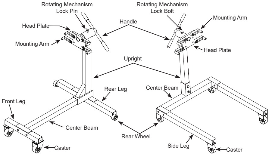
Figure 1 - Model 30750 Components
