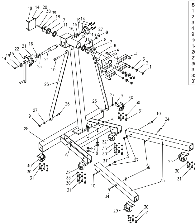
Figure 6 - Assembly Illustration for Model 31256
