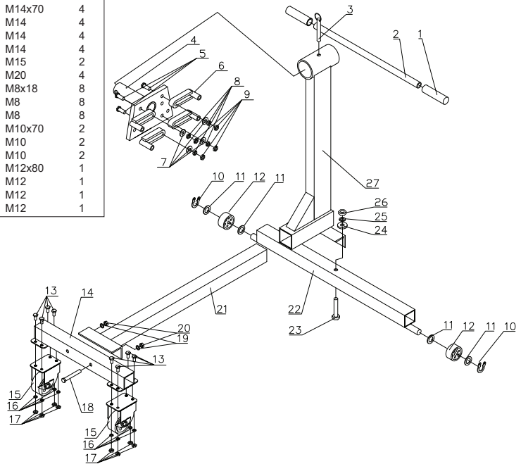
Figure 4 - Assembly Illustration for Model 30750
