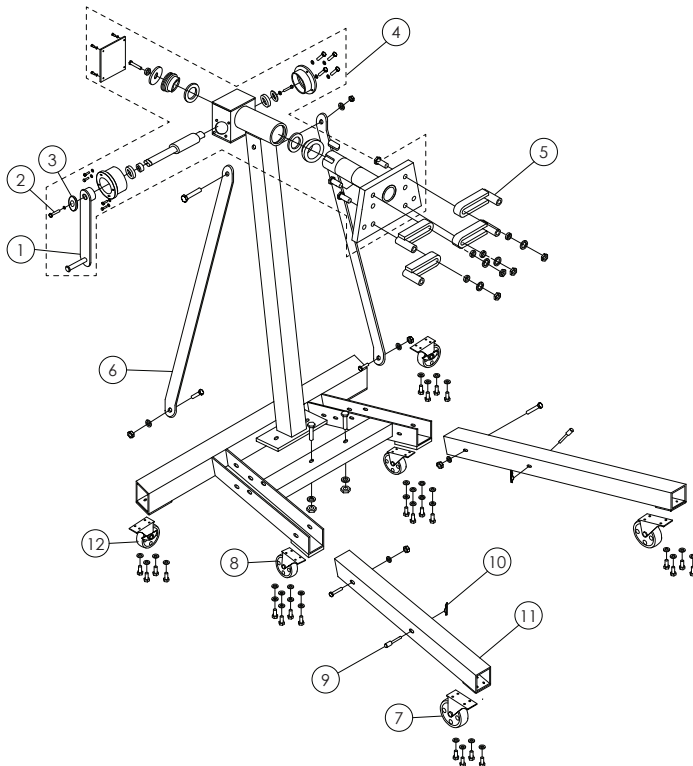
Figure 10 - Replacement Parts Illustration for model 31256
