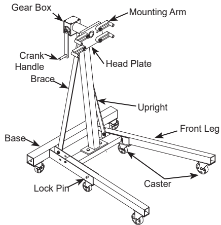
Figure 3 - Model 31256 Components
