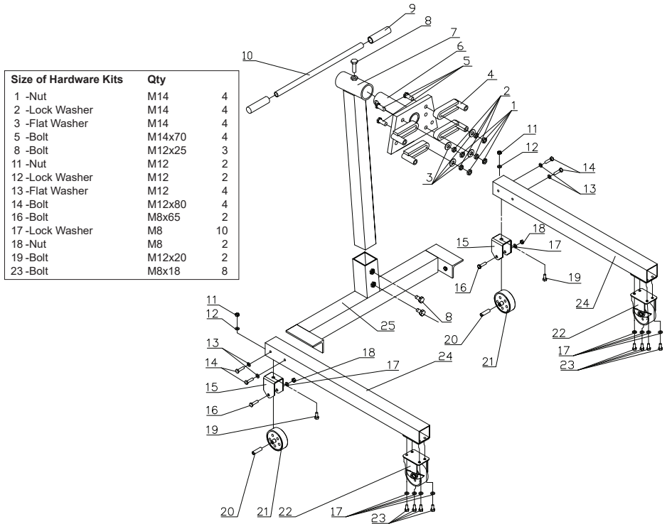
Figure 5 - Assembly Illustration for Model 31250
