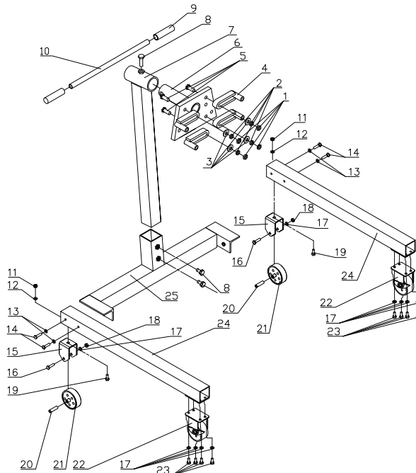
Figure 8 - Replacement Parts Illustration for model 31250
