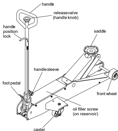
Figure 1 - Model 25057 & 25107 Components
