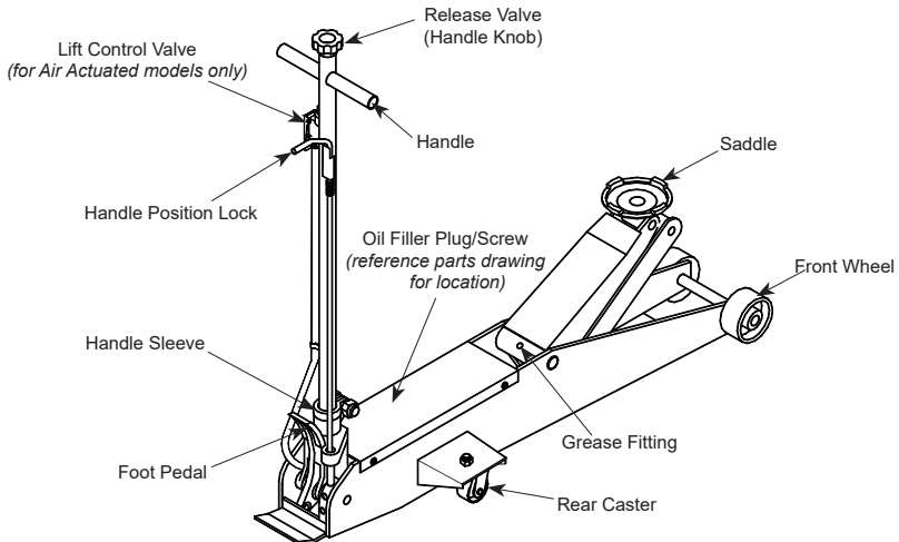
Figure 1 - Typical Long Chassis Jack Nomenclature (22051C shown)
