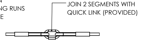
DETAIL B SCALE 1 : 4
