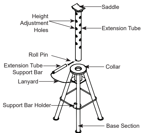
Figure 1 - Models 32105B & 32107B Components
