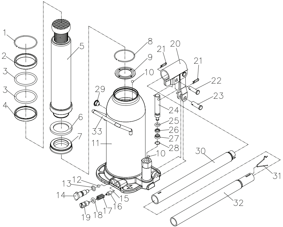
Replacement Parts Illustration for 10025W, 10045W, 10065W, 10125W, 10205W
