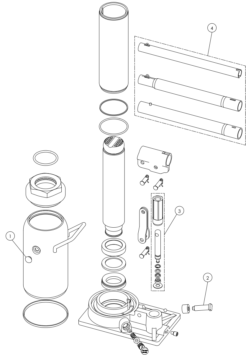
Figure 2 - Replacement Parts Illustration for Models 10120, 10128, 10200 & 10208
