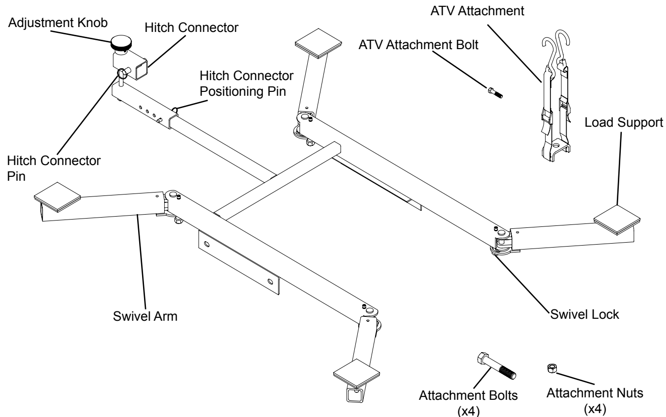
Figure 1 - Model T-2300AT Nomenclature
