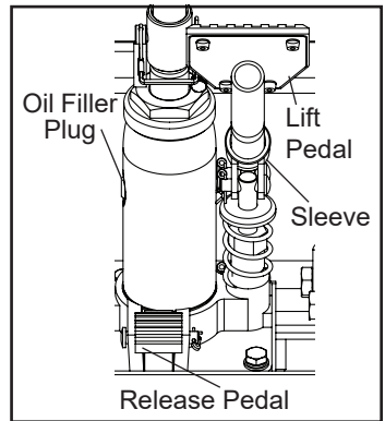
Hydraulic Unit
