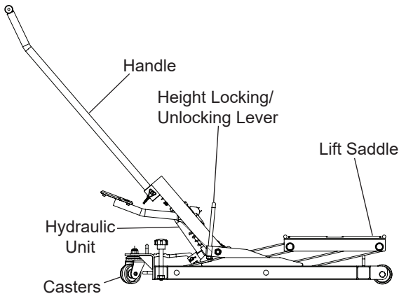
Figure 1 - Motorcycle/ATV Lift Nomenclature
