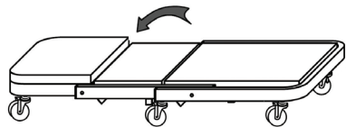
Figure 4 - Adjusting Seat to Creeper configuration
