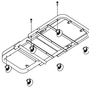
Figure 2 - Attaching Creeper Casters
