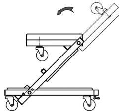
Figure 3 - Adjusting Creeper to seat configuration
