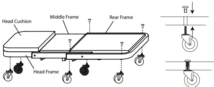
Figure 1 - Model B2036 Components
