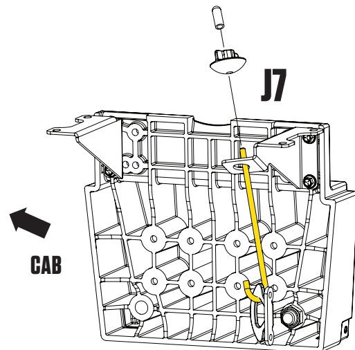
DRIVER SIDE CABSIDE CORNER SUPPORT
