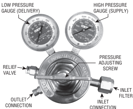
Figure 2: Pressure Regulator
