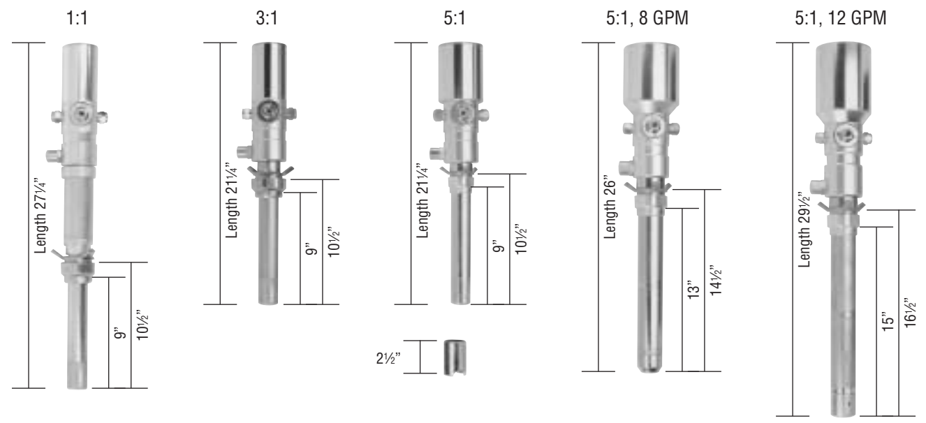
Extension pipe data chart
